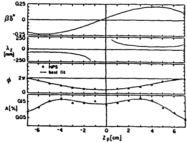
Fig. 4 Experimental HPS spanwise wavenumber, wave length, phase and maximum amplitude vs Z , F=104 at R_{\delta^*}=990 ( X_s=35 cm).
