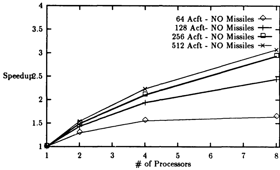
Figure 6.2. Simulation Speedup - without Missiles
