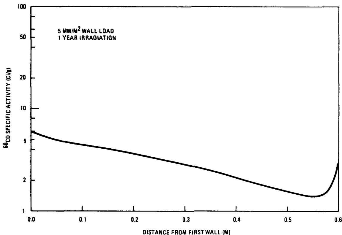
FIG. 6-8. Spatial distribution of 60 Co specific activity (Ci/g in a Li 17 Pb 83 blanket) (one year continuous operation at 5 MW/m 2 neutron wall loading.)
