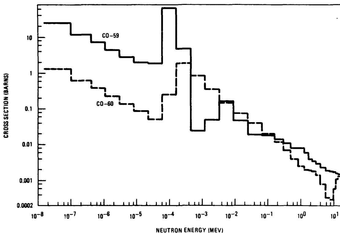
FIG. 6-3. Cobalt-59 and ^{60}\text{Co} ( n,\gamma ) evaluated cross sections.
