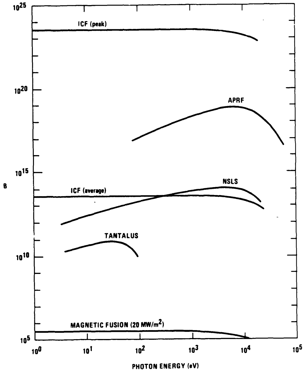
FIG. 13-3. Spectral brilliance B (photon/s) (\text{mm} \cdot \text{mrad})^2 (0.1% bandwidth) of some existing (Tantalus, National Synchrotron Light Source [NSLS]) and a proposed (Advanced Photon Research Facility [APRF]) synchrotron radiation sources. Also shown are estimated fusion bremsstrahlung at Z_{\text{eff}}=10 for ICF (peak and average) and magnetic fusion at 20 \text{ MW/m}^2 wall power.
