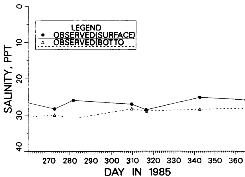
Figure B2. (Sheet 3 of 3)
