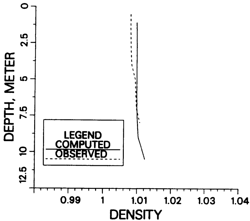
Figure B62. Comparison of vertical density profile at sta CB 3.3W during 1985 (Sheet 1 of 10)
