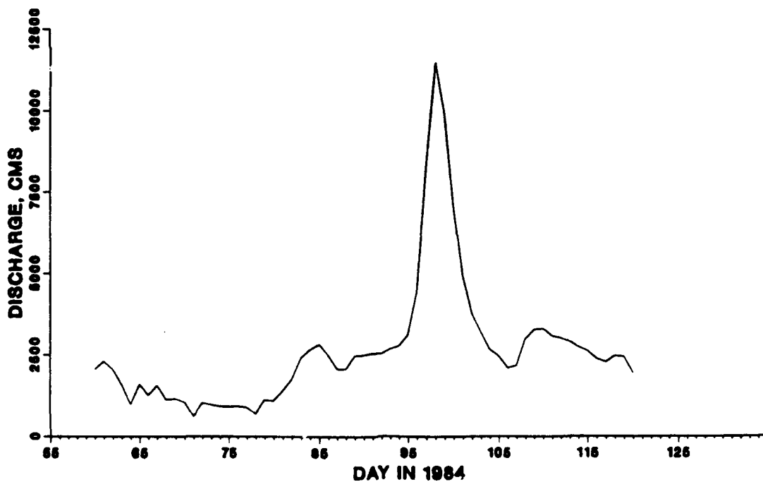
Figure A12. Freshwater inflow on Susquehanna River during 1984 (Sheet 1 of 3)
