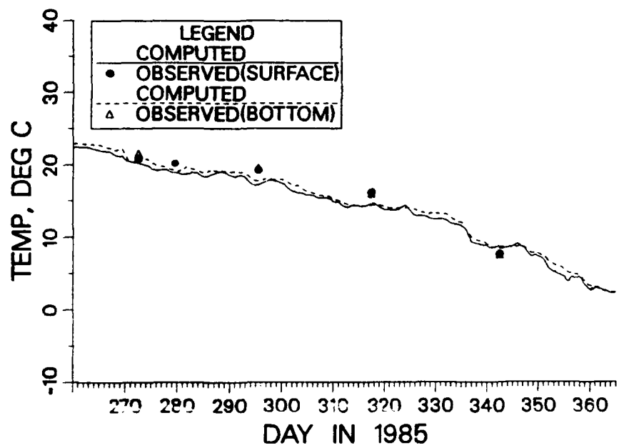
Figure B41. (Sheet 3 of 3)
