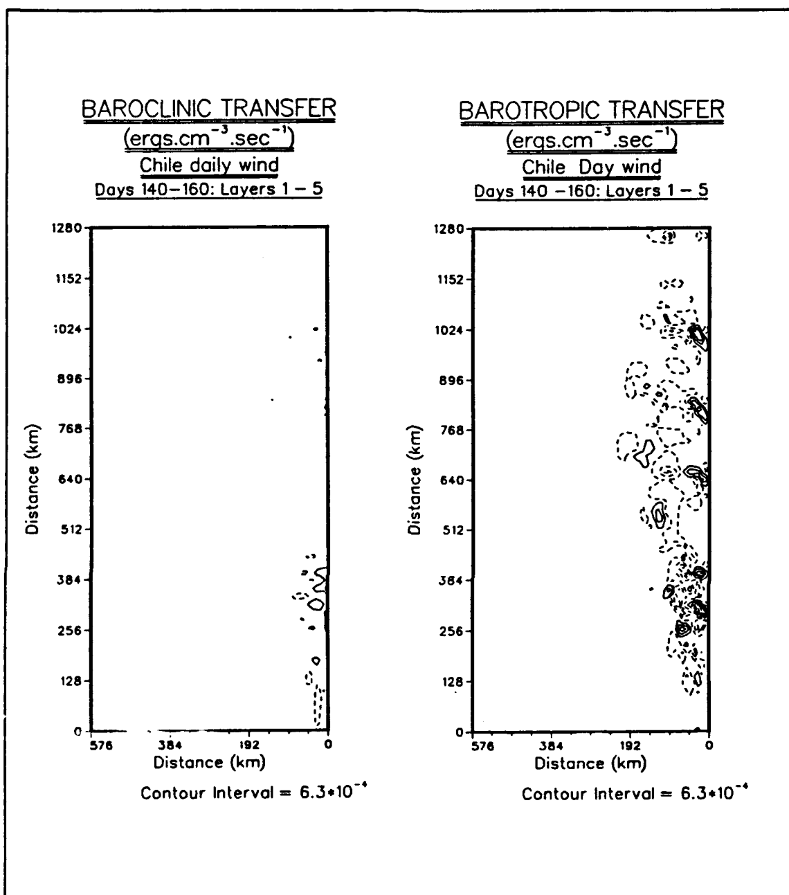
Figure 28. Baroclinic and barotropic instability at day 140 of Experiment 2.
