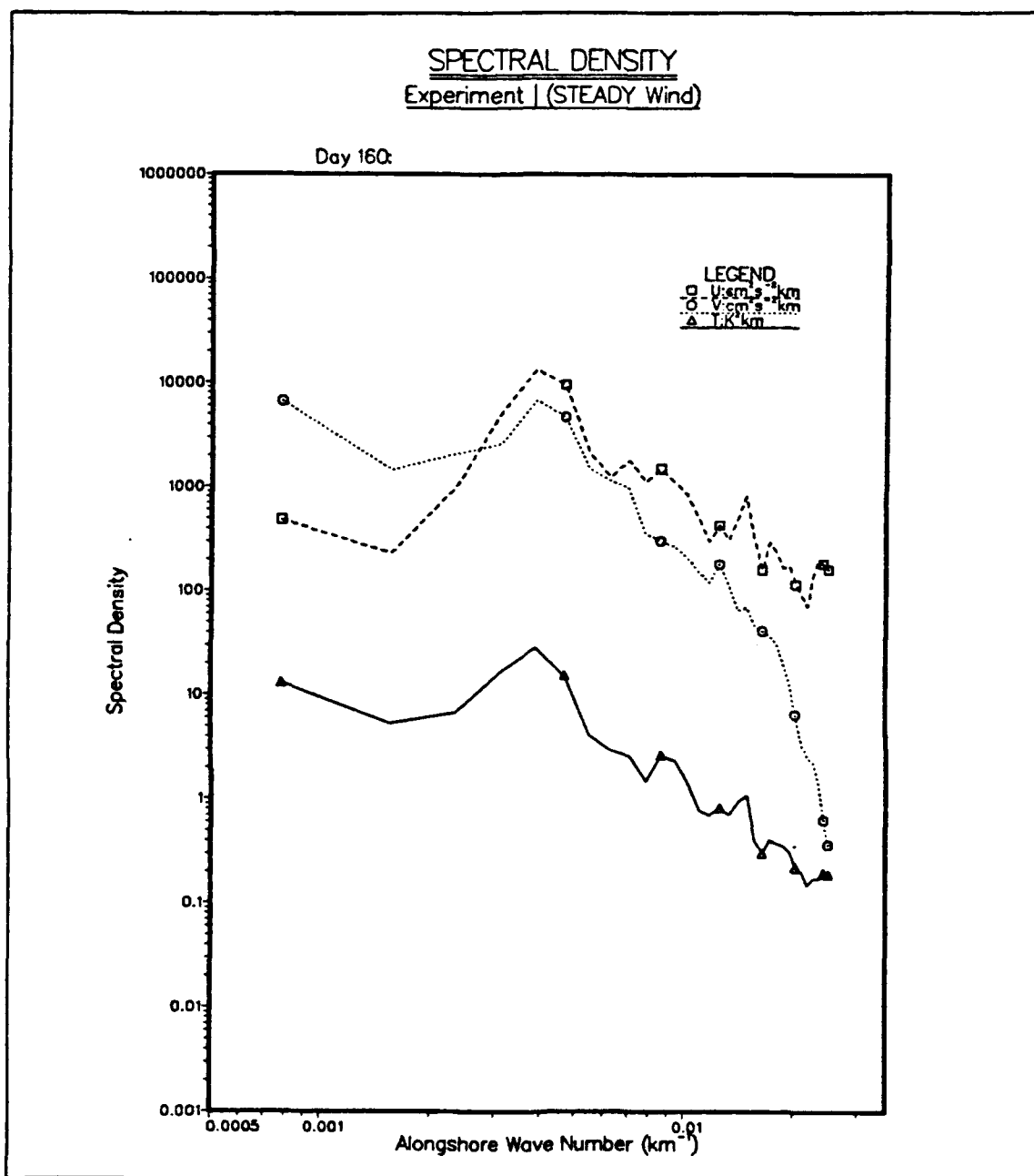
Figure 18. Spectral density at day 160 of Experiment I: Dominant wavelength is \sim 250 \text{ km} .
