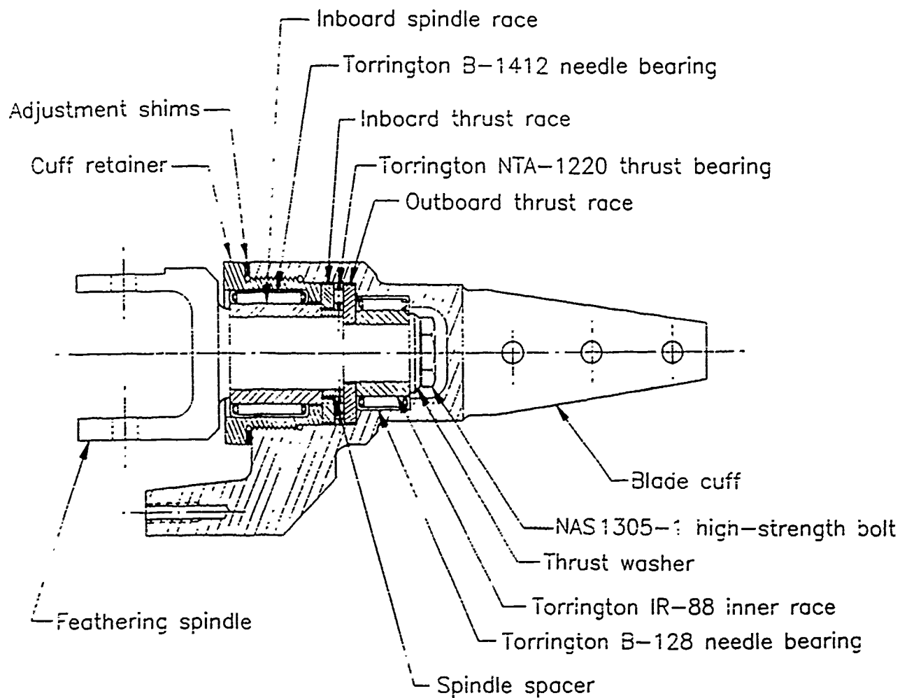
Figure 2. Sketch of Blade Cuff Assembly
