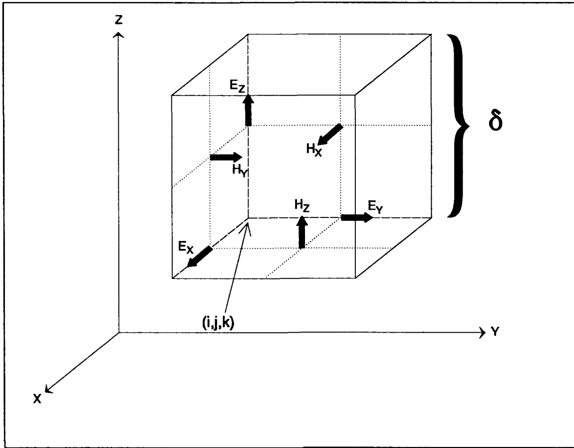
Figure 1 -- Yee Cell
