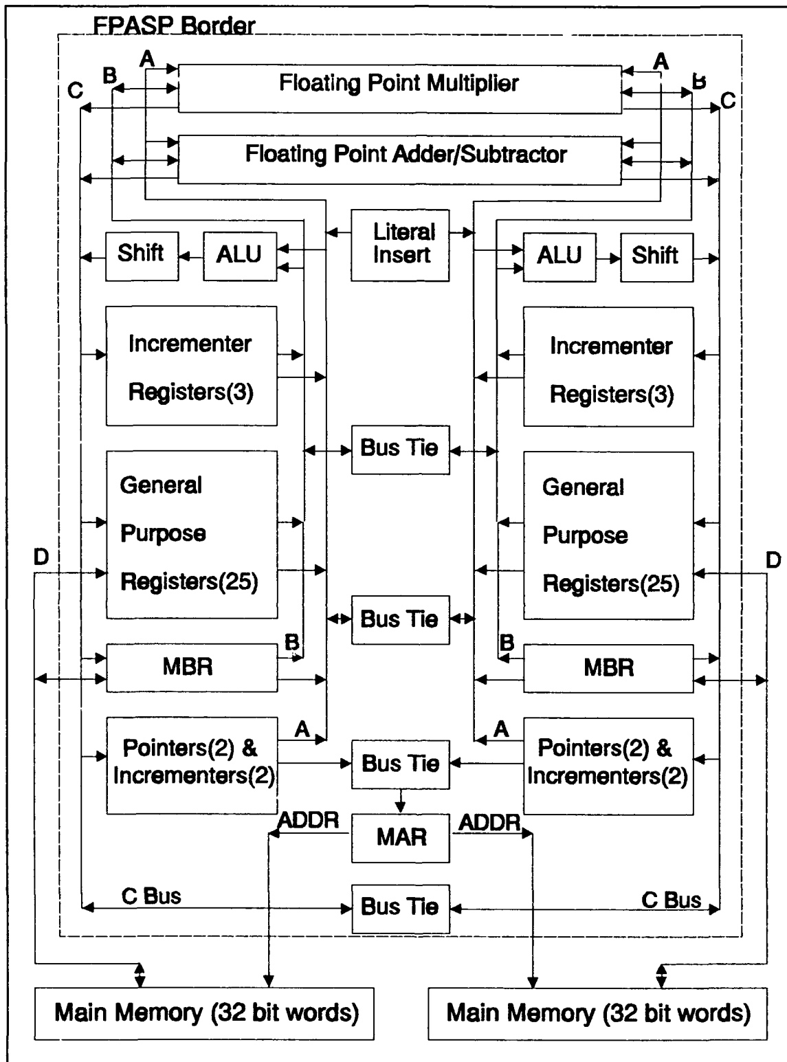
Figure 5 -- FPASP Architecture
