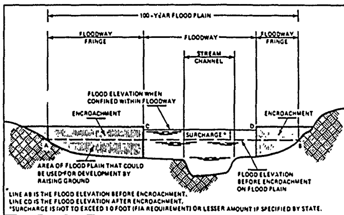
Figure 2 - Floodway Schematic
