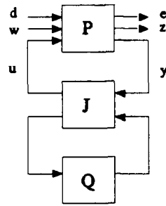
Figure 6-1. Mixed Optimization Block Diagram with Q(s)
