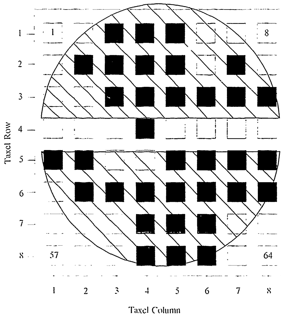
Figure 6.45. 0.51-V Threshold Plot Of A 100 g Slotted Screw Shaped Load - Taxels With An Output Level Above This Threshold Level Are Displayed As Black And Taxels With An Output Level Below This Threshold Level Are Displayed As White.
