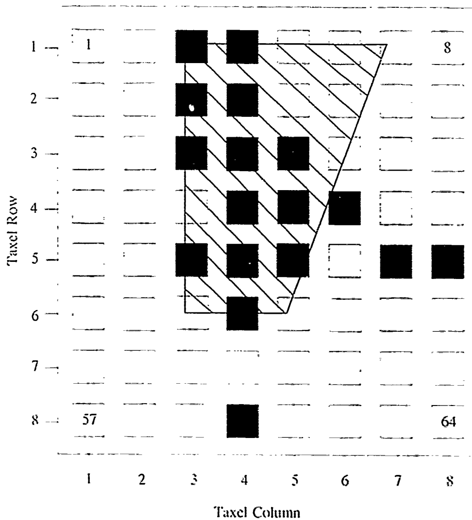
Figure K.36. 0.6-V Threshold Plot Of A 10 g Potygon Shaped Load Taxels With An Output Level Above This Threshold Level Are Displayed As Black And Taxels With An Output Level Below This Threshold Level Are Displayed As White.
