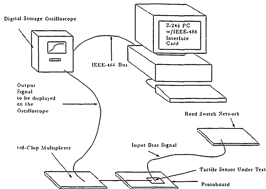
Figure 5.6. Tixel Array Evaluation Instrumentation Arrangement.
