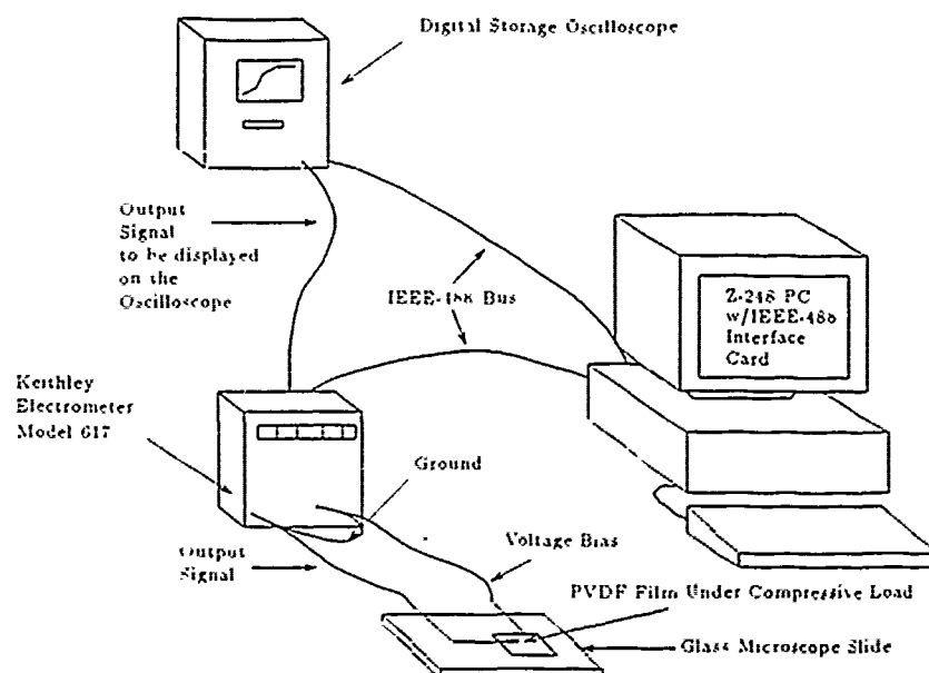
Figure D.2. Piezoelectric PVDF Film Characterization Instrumentation Configuration.
