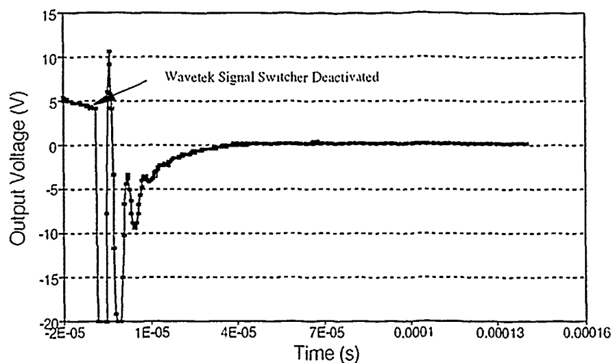
Figure 6.15. The Output Of The Wavetek Signal Switcher Connected To The Reed Switch Control Line.
