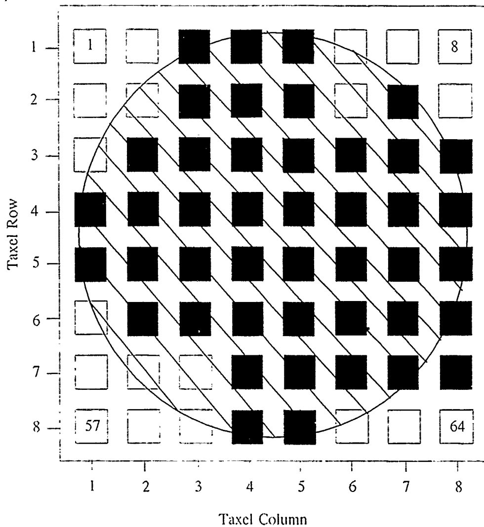
Figure 6.51. 0.5-V Threshold Plot Of A 100 g Large Solid Circularly Shaped Load - Taxeis With An Output Level Above This Threshold Level Are Displayed As Black And Taxels With An Output Level Below This Threshold Level Are Displayed As White.
