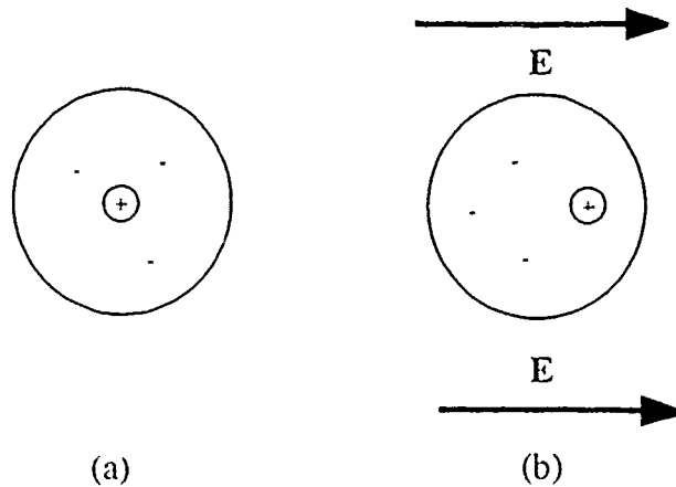
Figure 3.2. Model Of An Atom: (a) Without An External Electric Field Present. And (b) The Resulting Atomic Dipole After An External Electric Field E Is Applied (66:60).
