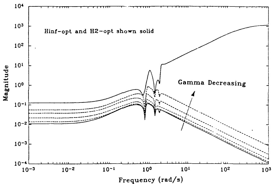
Figure 6.7 \sigma -Plot of the Mixed Controllers
