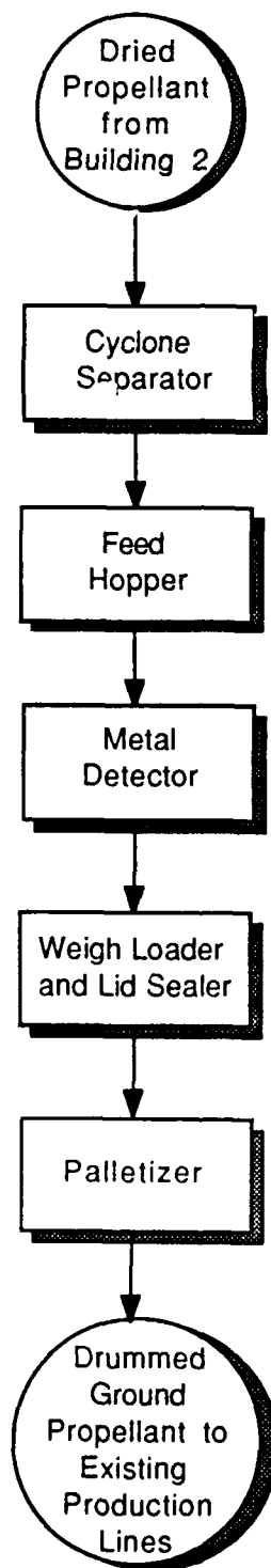
FIGURE 2.3 SCHEMATIC FLOW DIAGRAM FOR PROPELLANT GRINDING (BUILDING 3)
