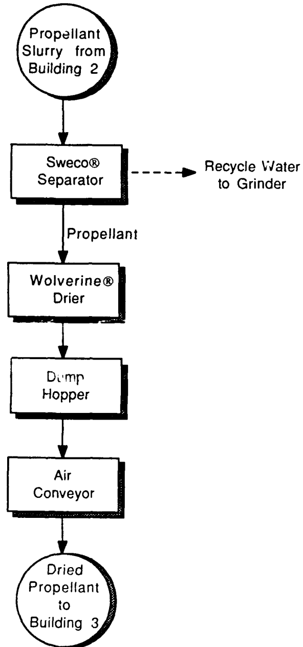
FIGURE 2.2 SCHEMATIC FLOW DIAGRAM FOR PROPELLANT GRINDING (BUILDING 2)
