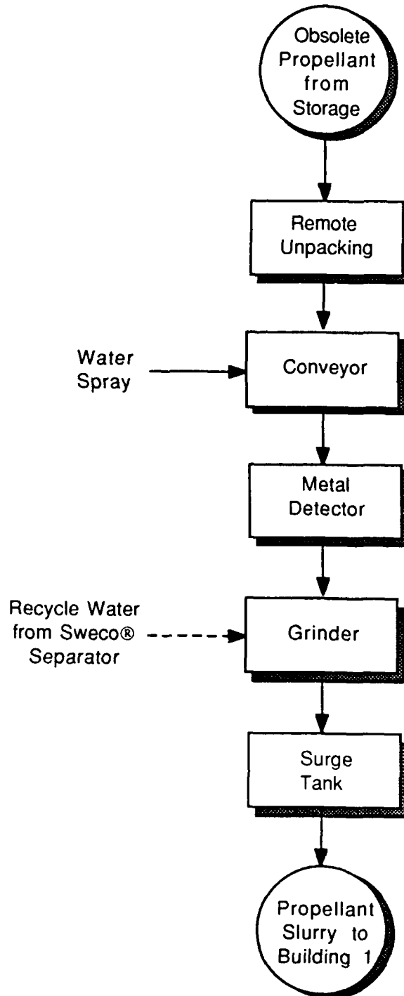
FIGURE 2.1 SCHEMATIC FLOW DIAGRAM FOR PROPELLANT GRINDING (BUILDING 1)
