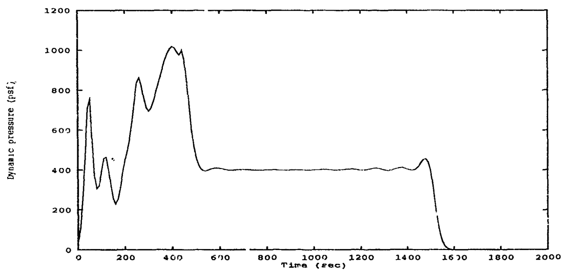
Figure 42. Baseline Trajectory Dynamic Pressure versus Time.
