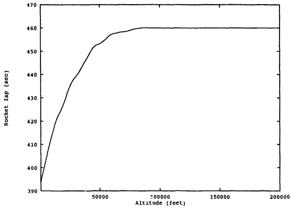
Figure 38. Rocket Fuel Specific Impulse (8:23-24).
