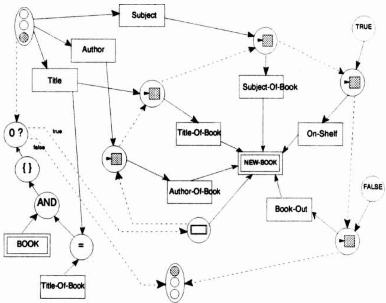
Figure H.1. Visual Refine: Add-Book-To-Library
