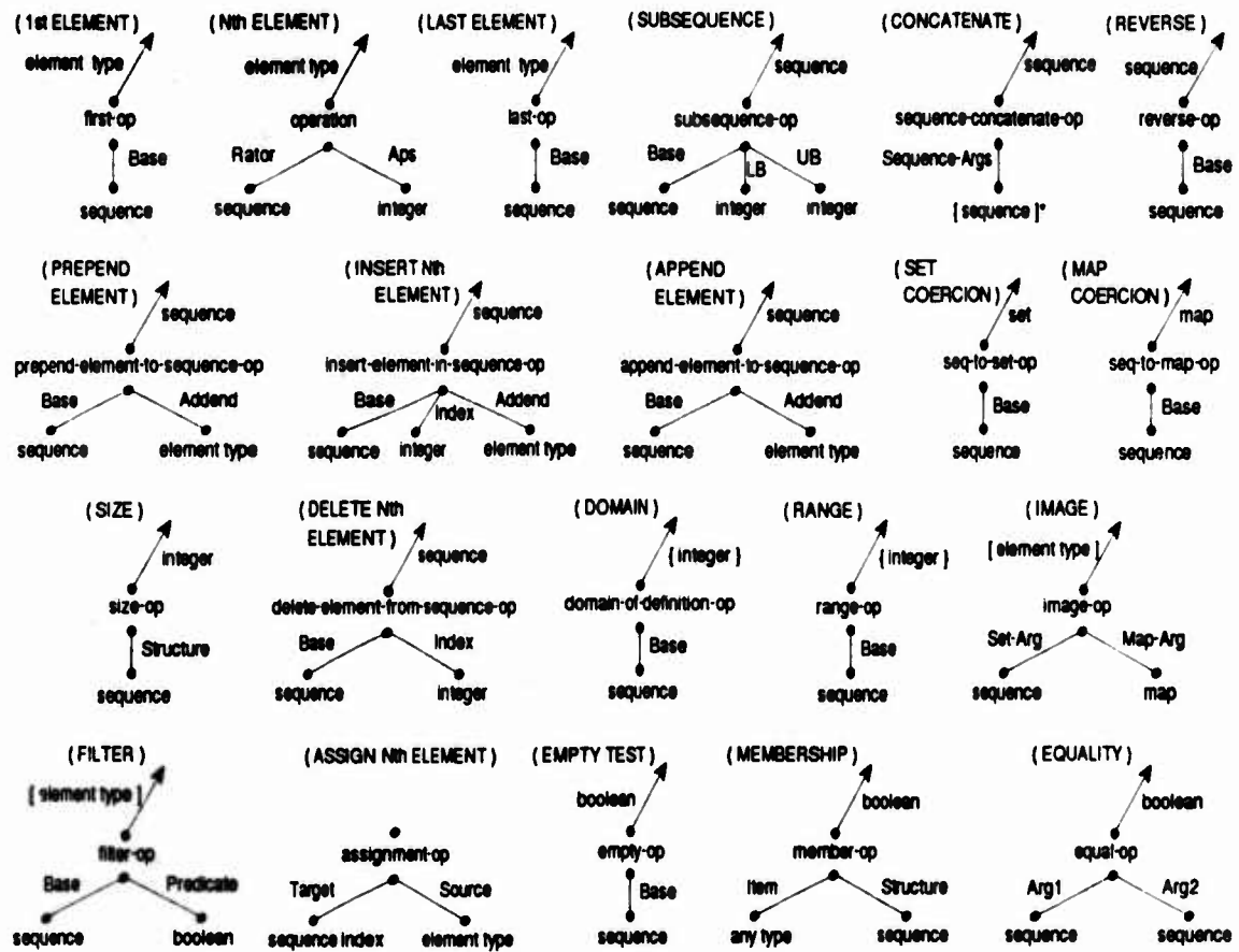
Figure D.5. Sequence Operations
