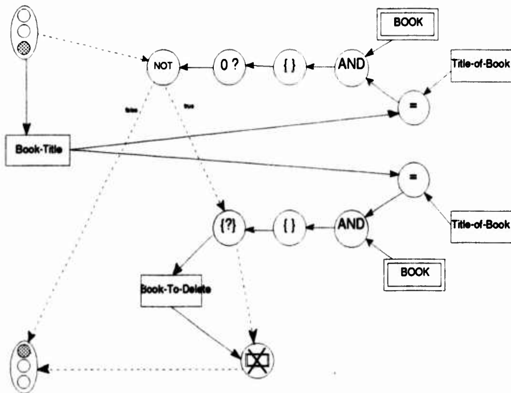
Figure H.2. Visual Refine: Remove-Book-From-Library
