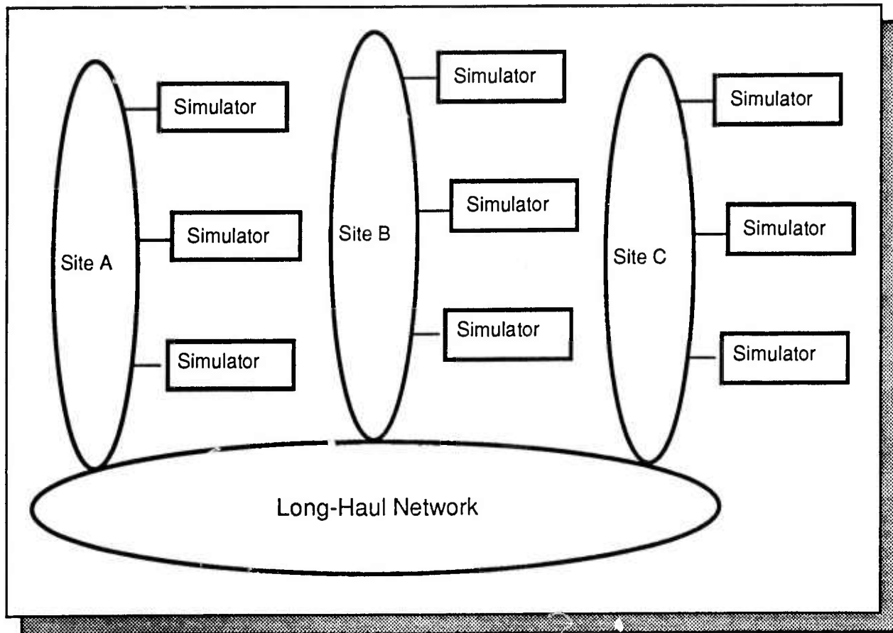
Figure 2-1 SIMNET Architecture.
