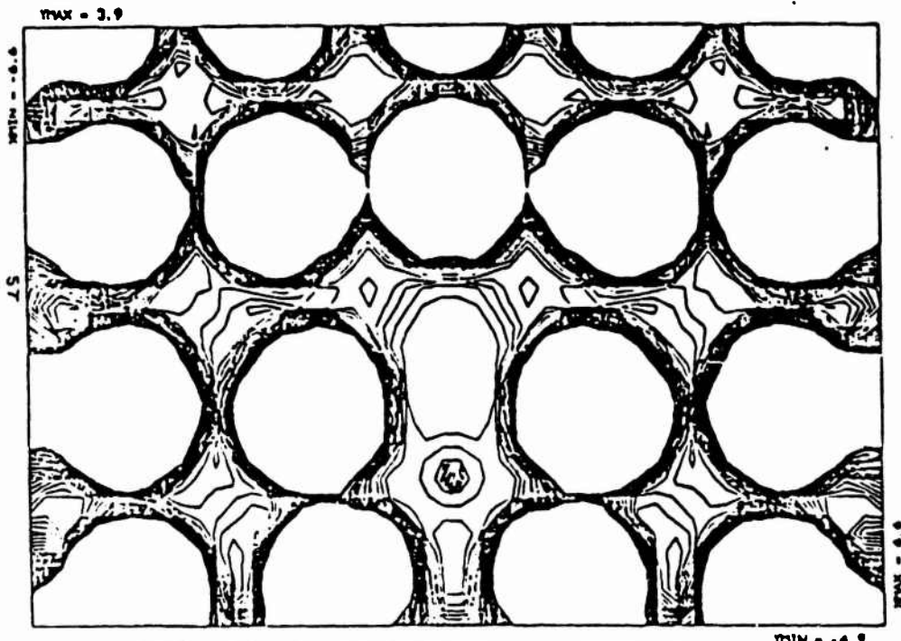
Fig. 6(a). Contour energy plot of hydrogen in region of gh shown in Fig. 6(b).
