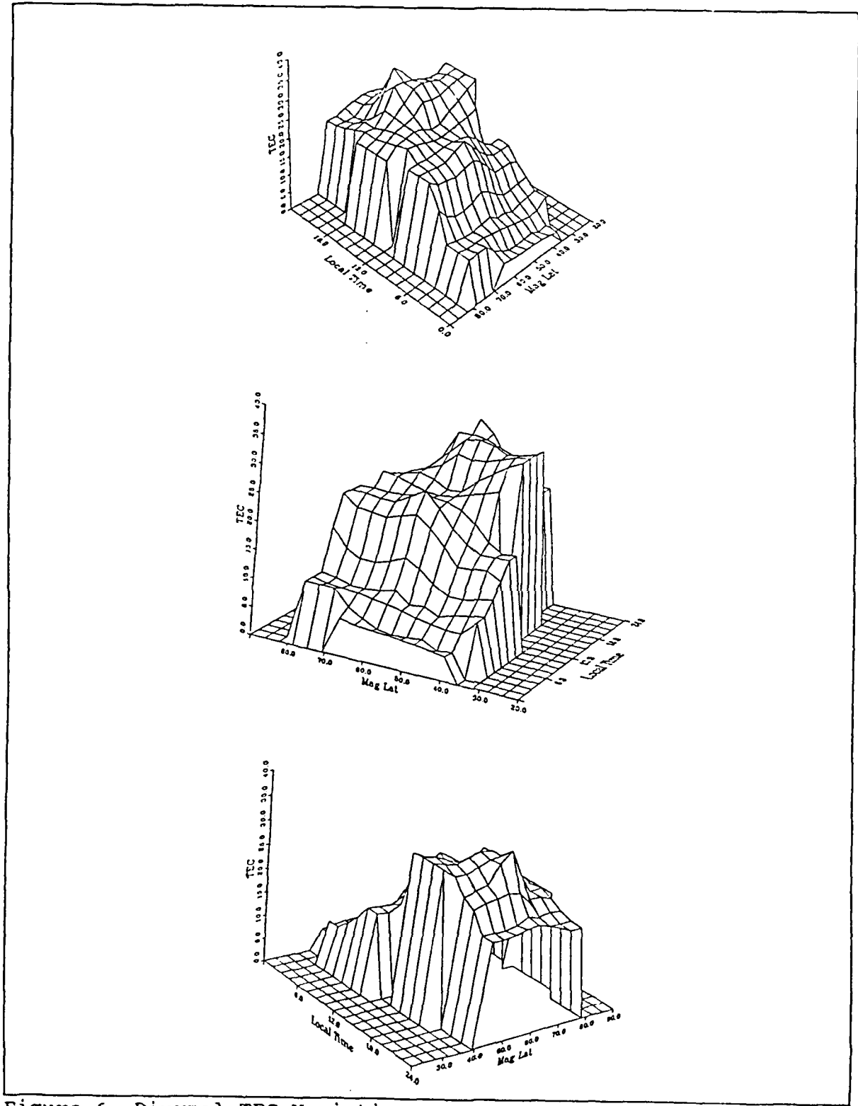
Figure 6. Diurnal TEC Variation
