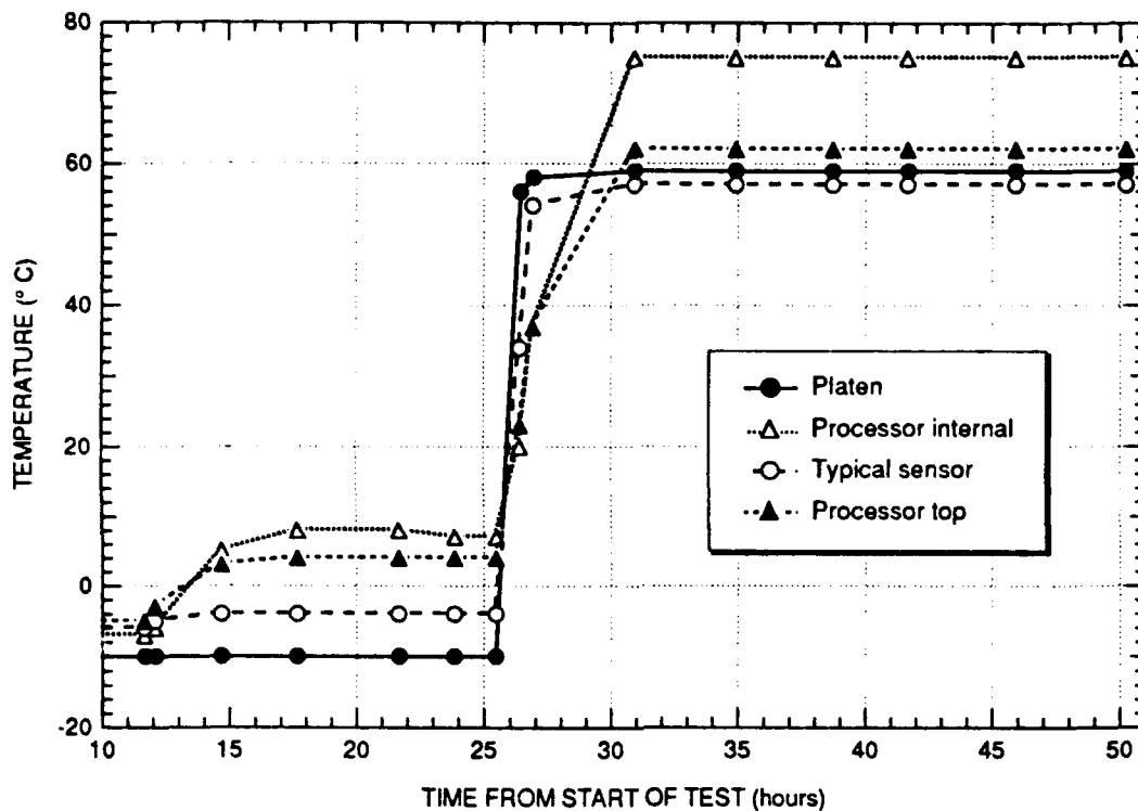
Figure 13. Temperature During Vacuum Tests.
