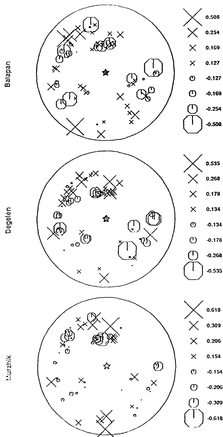
Figure 4. Lower-hemisphere equal-area projection of station-corrected m_b(P_{max}) anomalies for Soviet's 3 test sites in Eastern Kazakhstan. For each station, the mean m_b anomaly is defined as the mean residual averaged over all explosions from the same test site. The different patterns more or less reflect the focusing/defocusing underneath the source region.
