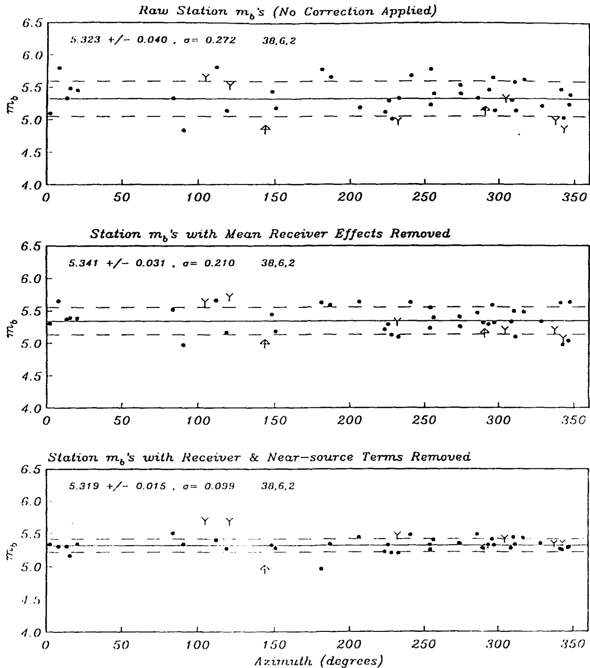
Figure 6. Scatter plot of 3 different types of station m_b 's for Murzhik explosion 710606. The 38 good recordings, 6 noise, and 2 clips are shown with filled circles, Y-shaped downward arrows, and upward arrows, respectively. The raw station m_b 's (top) has a standard deviation of 0.27 m.u. Applying the "primary" station corrections reduces the scatter to 0.21 m.u. Applying the proposed "secondary" station corrections to count for the near-source focusing/defocusing effects would further reduce the scatter down to 0.1 m.u. The dashed lines around the network-averaged m_b clearly illustrate the remarkable reduction of fluctuation across the recording stations. The mean event m_b itself is not significantly changed, however.
