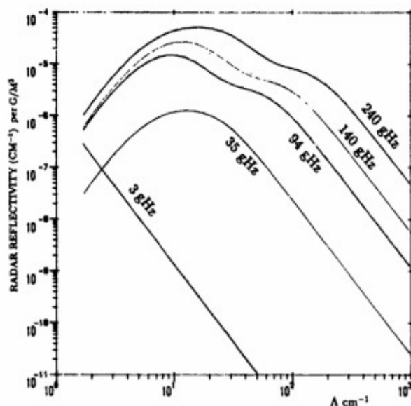
FIG. 10. Radar reflectivity at the indicated radar frequencies of a medium composed of hailstones with an exponential size distribution N = N_0 \exp(-AD) , as a function A . The radar reflectivity based on Rayleigh scattering at 3 GHz is also shown.
