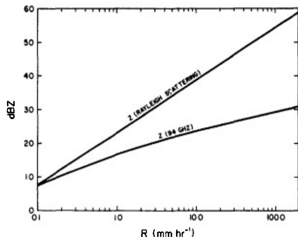
FIG. 10. Radar reflectivity factor, Z , as a function of rainfall rate for a long-wavelength radar (Rayleigh scattering) and a 94-GHz radar. Marshall-Palmer dropsize and the Gunn-Kinzer vertical velocity/diameter relationship are used.
