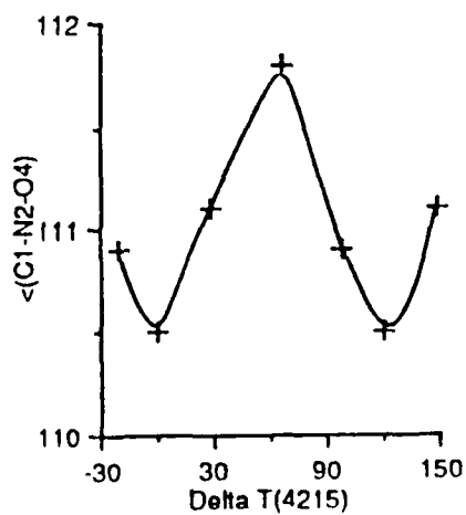
FIGURE 7-6 C1-N2-O4 ANGLE
