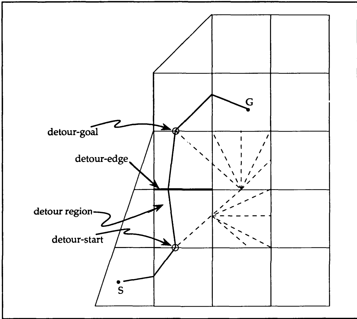
Figure 16. Finding a Detour
