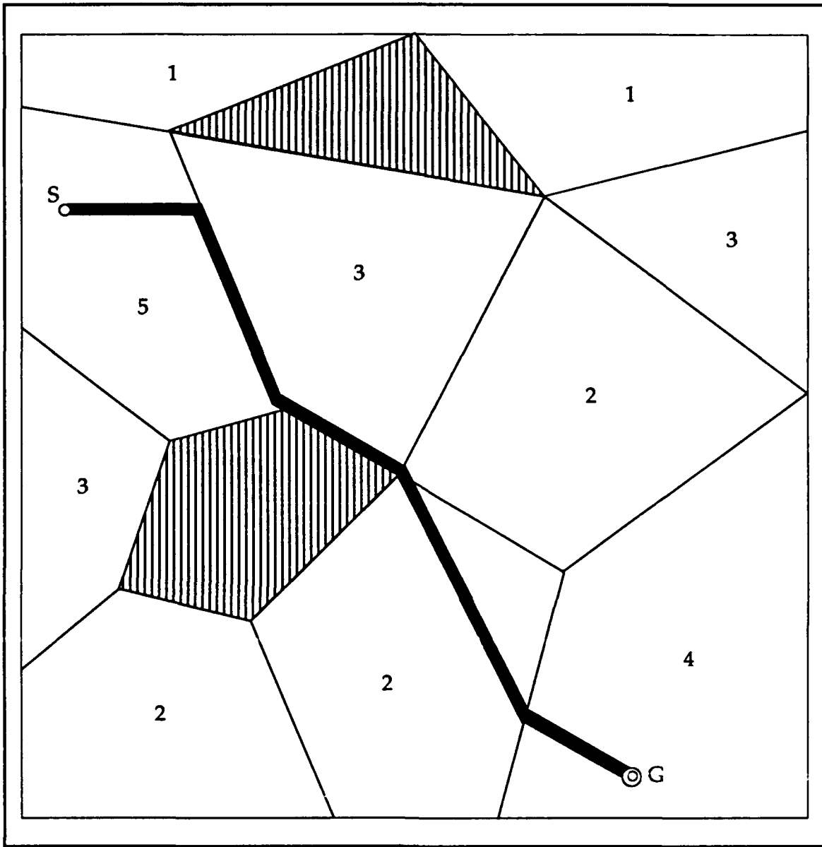
Figure 1. Weighted Region Problem
