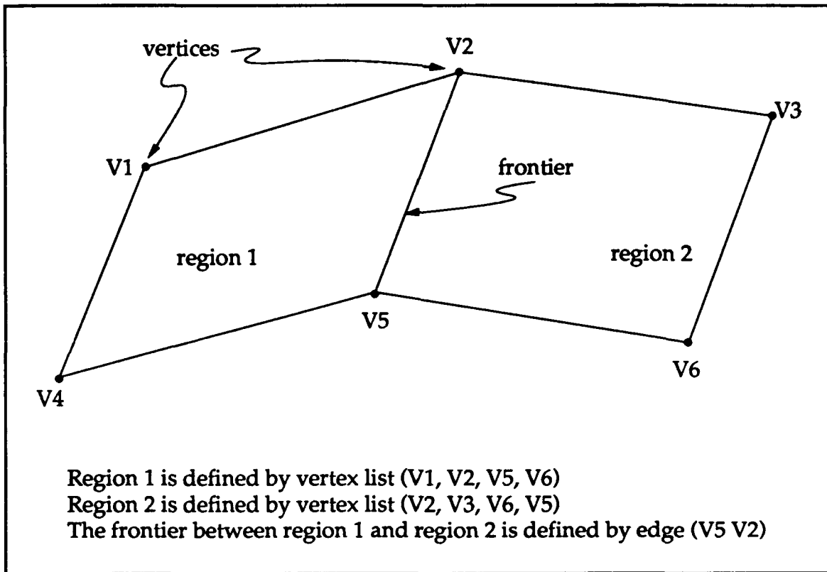
Figure 6. Regions, Vertices, and Frontiers
