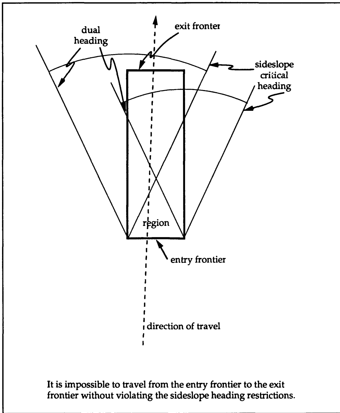
Figure 10. Narrow Region with Nonpermissible Entry
