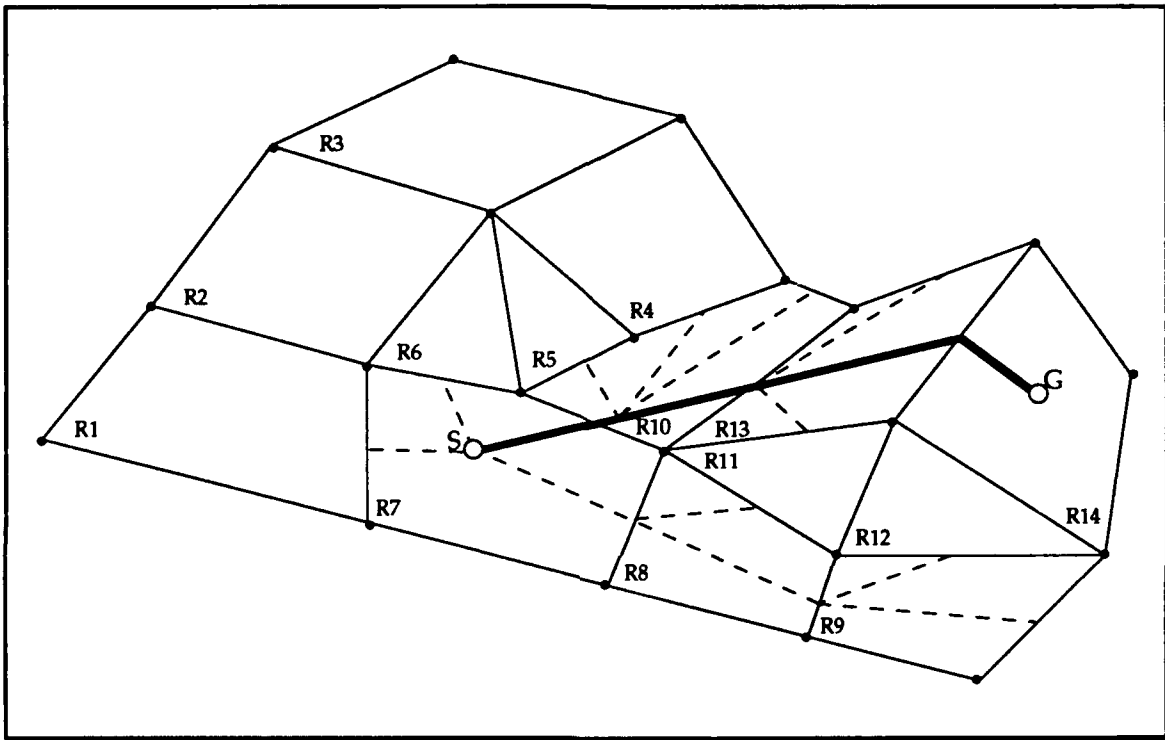
Figure 9. A* Search
