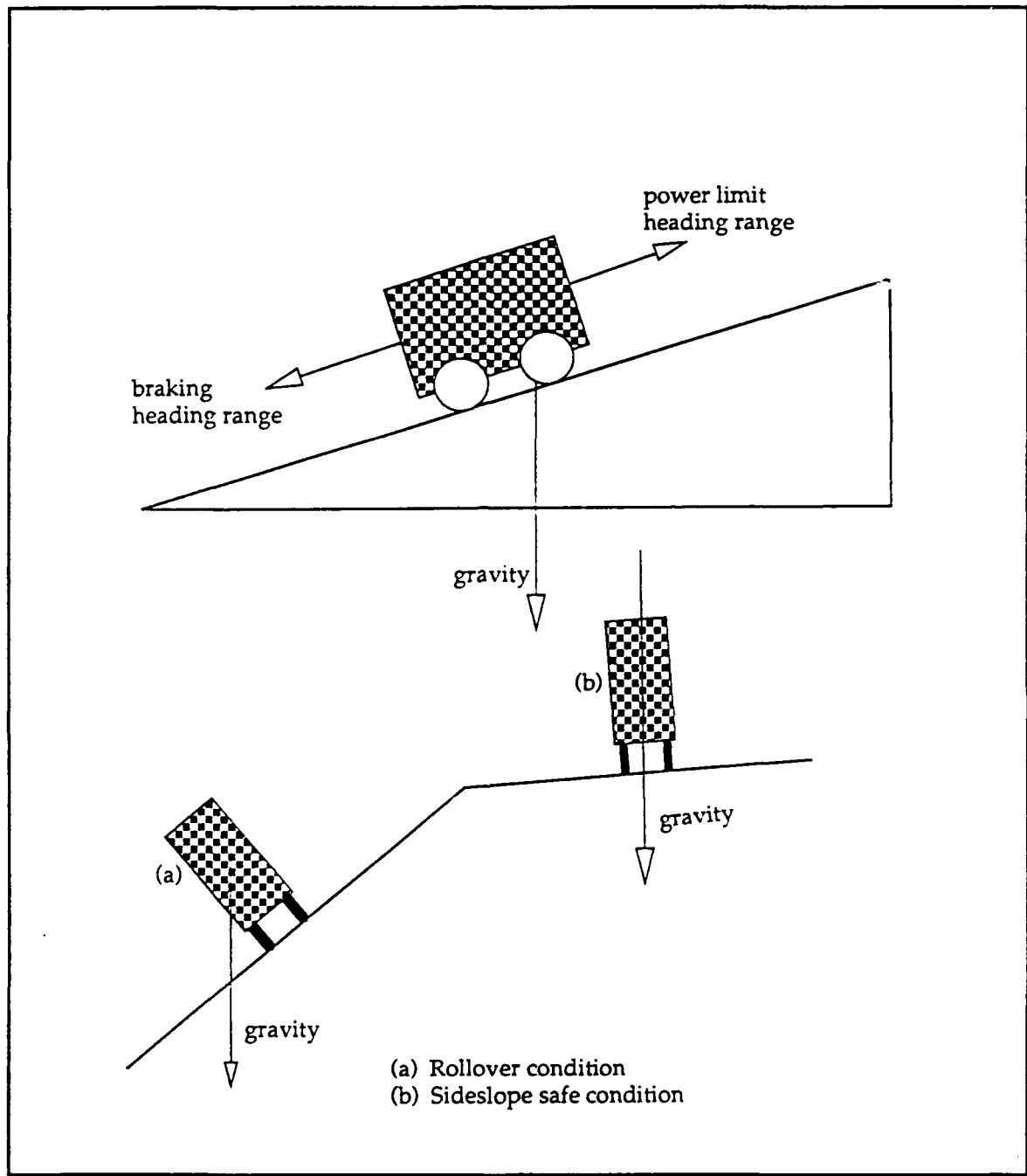
Figure 4. Vehicle Model
