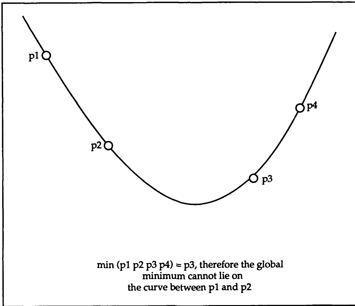
Figure 12. Golden Ratio Search
