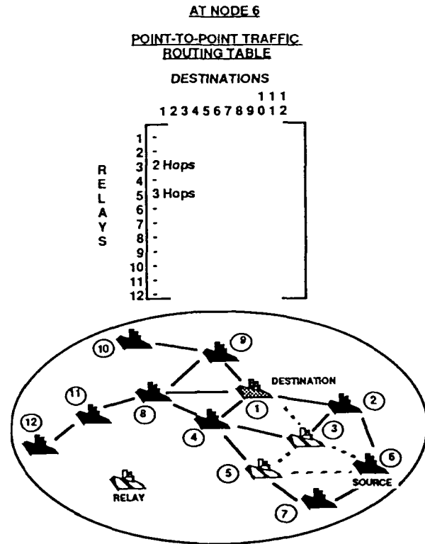
Figure 5 BACKWARDS LEARNING POINT-TO-POINT ROUTING
