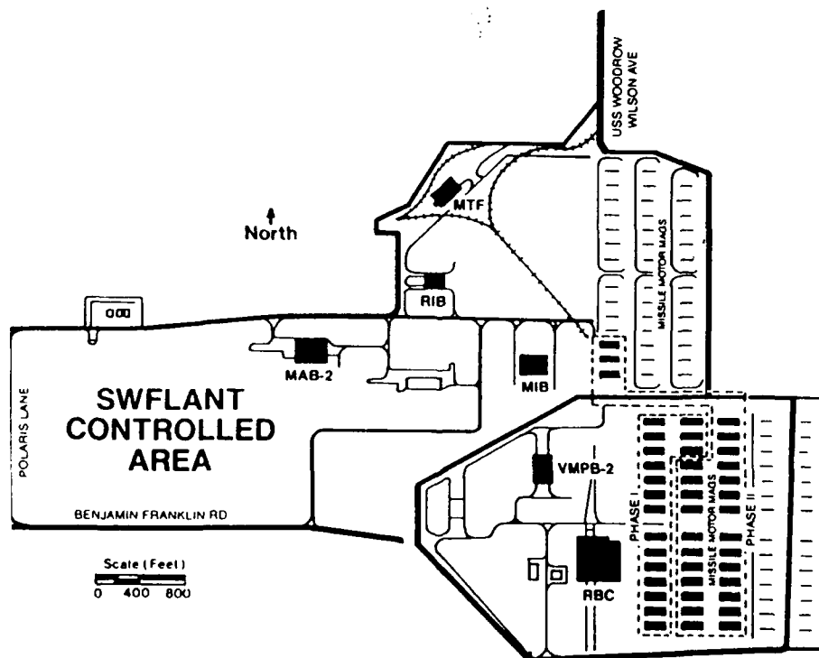
Figure 30. Site Plan of SWFLANT Area. (Hussin, 1987)
