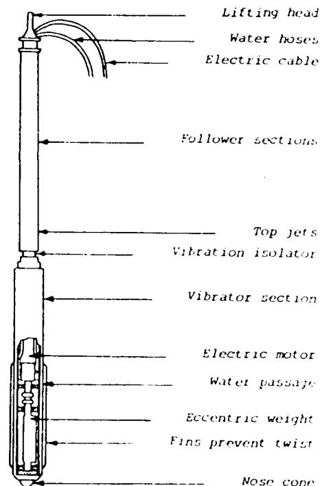
Figure 1. Essential features of the Vibroflot. (Glover, 1982)
