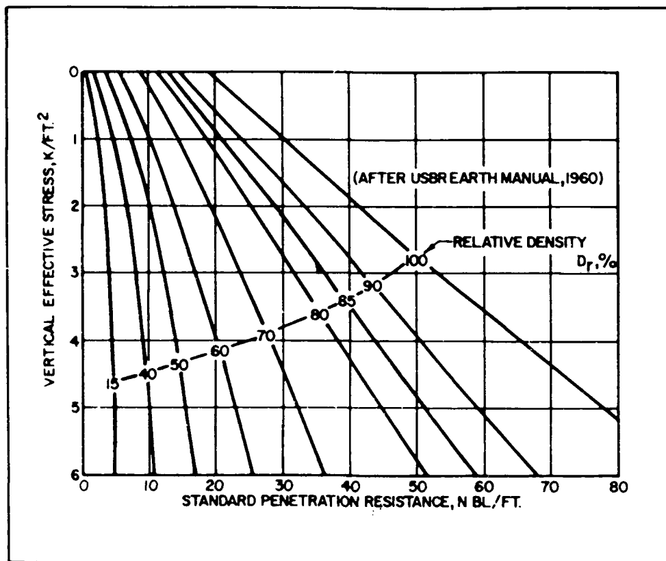
Figure 13. Relative density versus standard penetration resistance. (NAVFAC DM 7.1)
