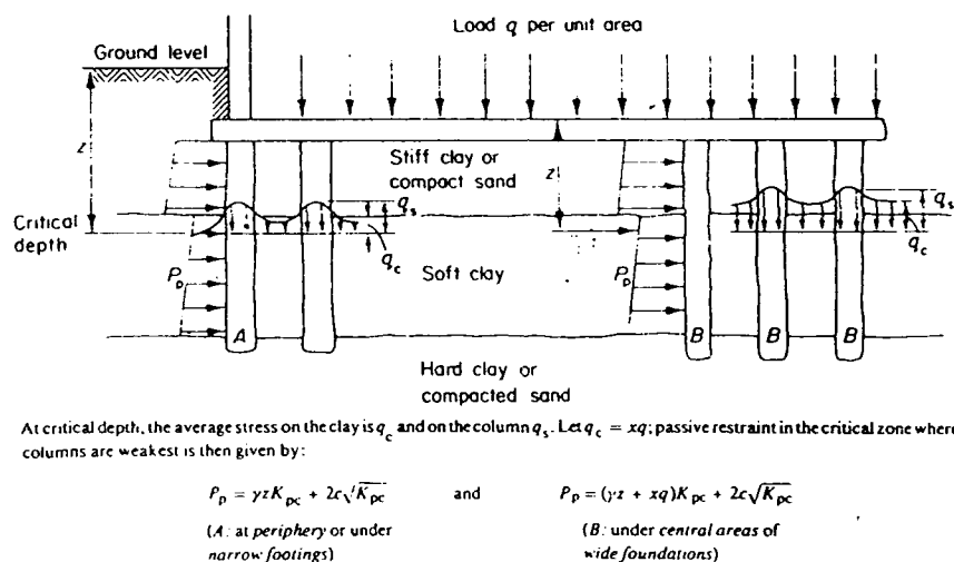
Figure 17. Stone Column Design - Passive Restraint. (Bell, 1975)
