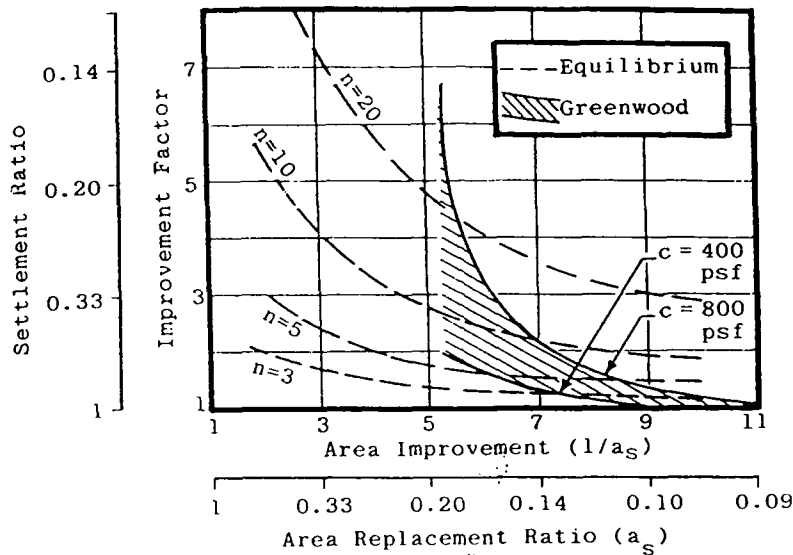
Figure 23 Comparison of methods for settlement reduction. (Bachus, 1989)
