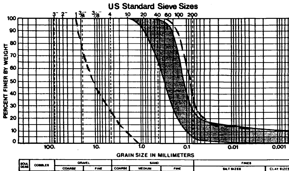
Figure 29. Range of soils densifiable by vibro-systems superimposed over the naturally occurring soil grain size distribution.
