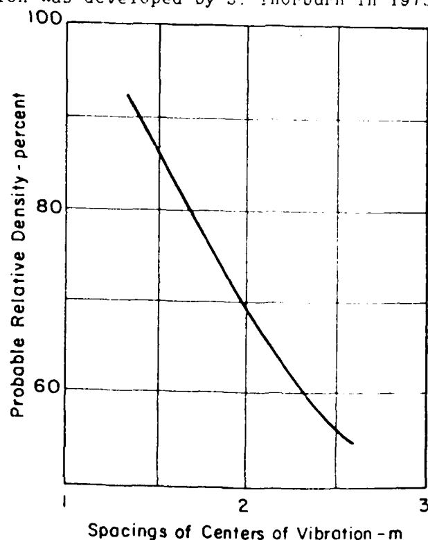
Figure 11. Relative density of clean sand as a function of probe spacing. (Thorburn, 1975)
