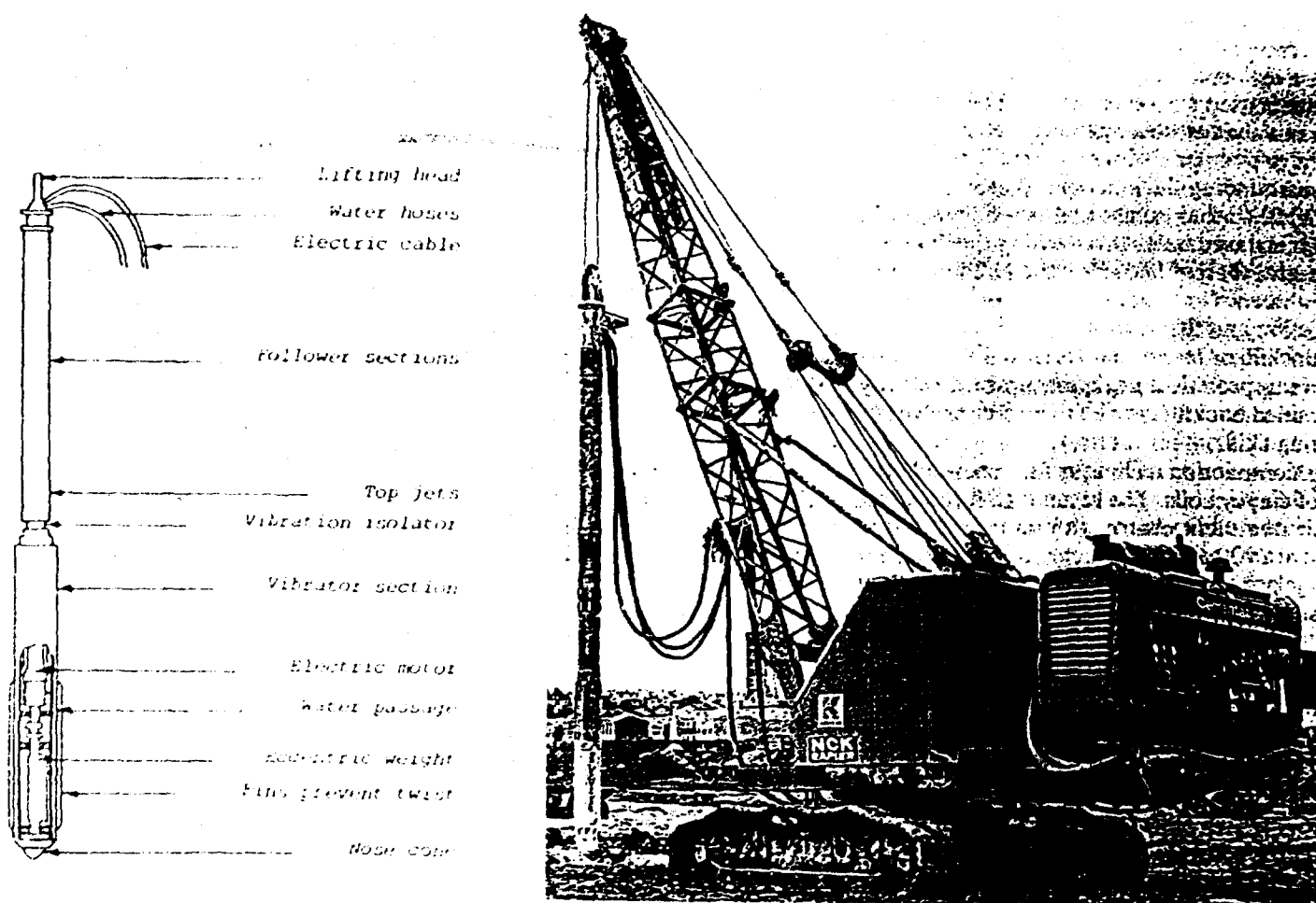
Figure 3. a.) Schematic drawing of the Vibroflot. b.) Field application of the Vibroflot. (Bell, 1975)
