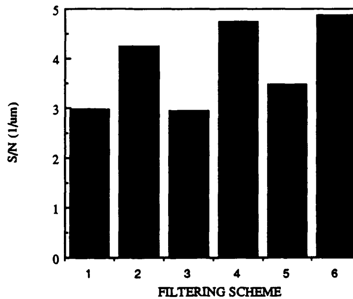
Fig 23: Signal to noise ratio vs filter combination for bifurcated coaxial cable with SMA end (uncollimated).
