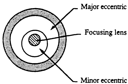
Fig 2: Eccentric coupler for coupling laser beam into illumination fiber.
