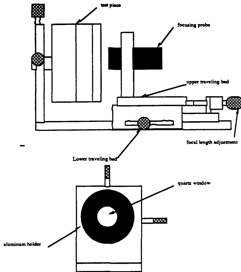
Fig 11: Bench testing apparatus.
