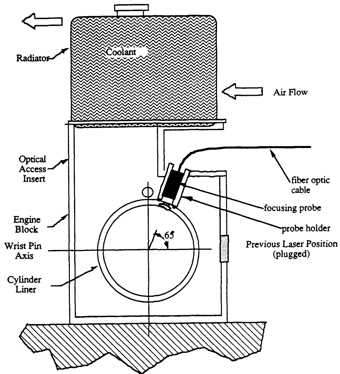
Figure 7: Modified engine.
