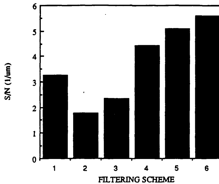
Fig 22: Signal to noise ratio vs filtering combination for bifurcated coaxial cable with SMA end (collimated).
