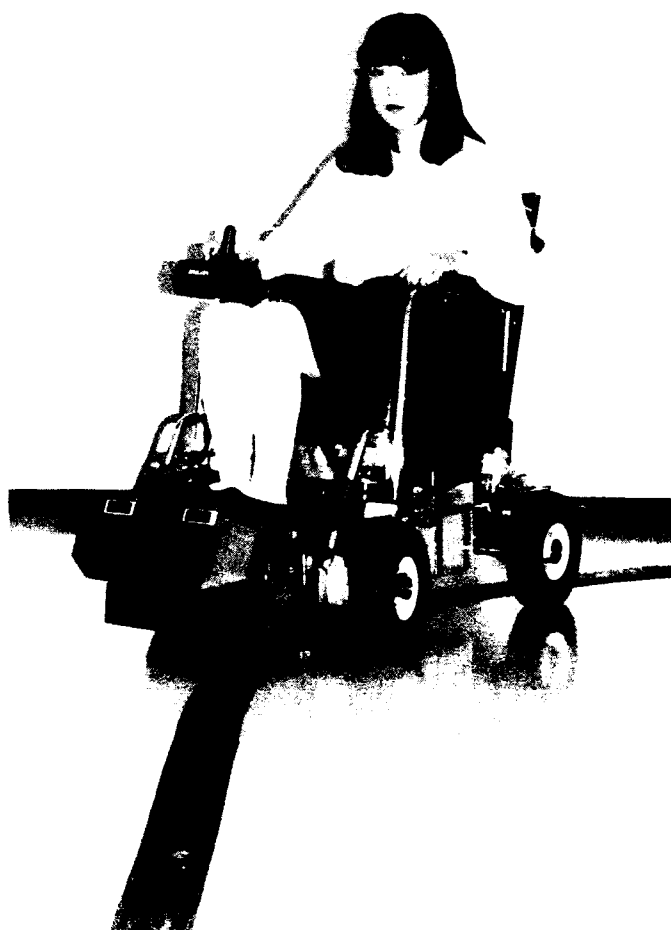
Figure 7. Automated wheelchair during running experiment. Two infrared obstacle detection sensors are installed at the front.
