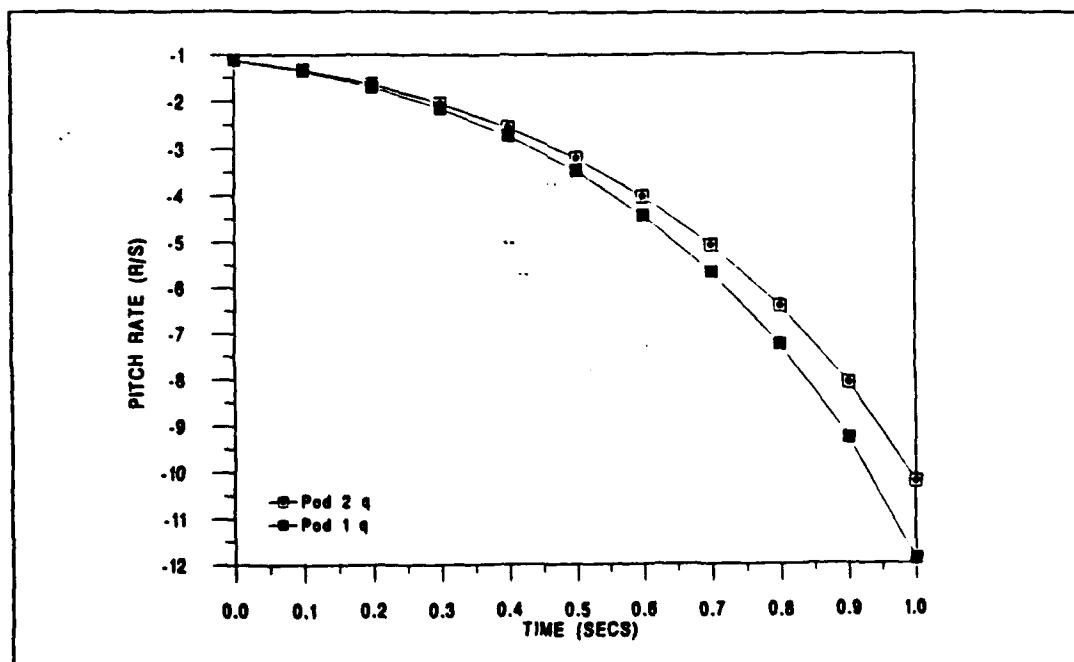
Figure 6 Pitch Rate Response
