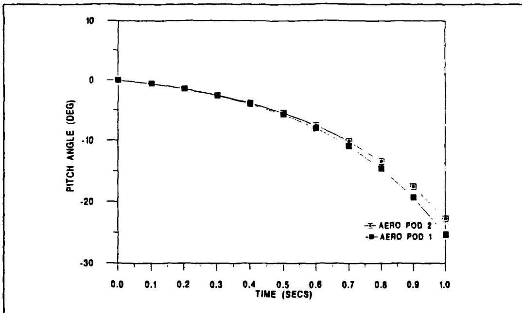
Figure 5 Pitch Angle Response
