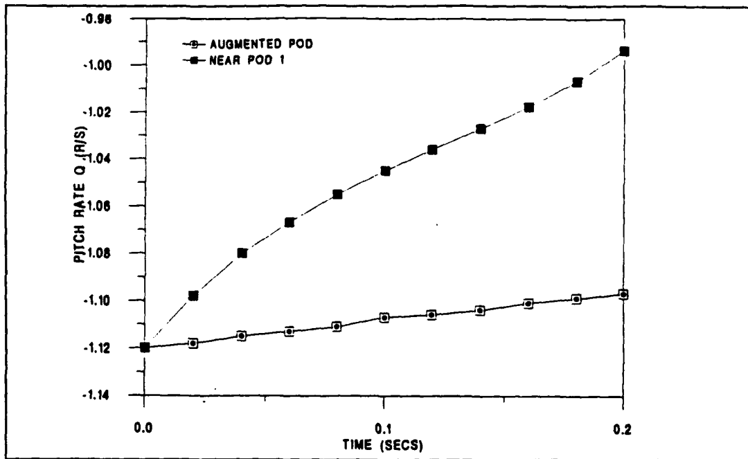
Figure 19 Pitch Rate (Augmented)
