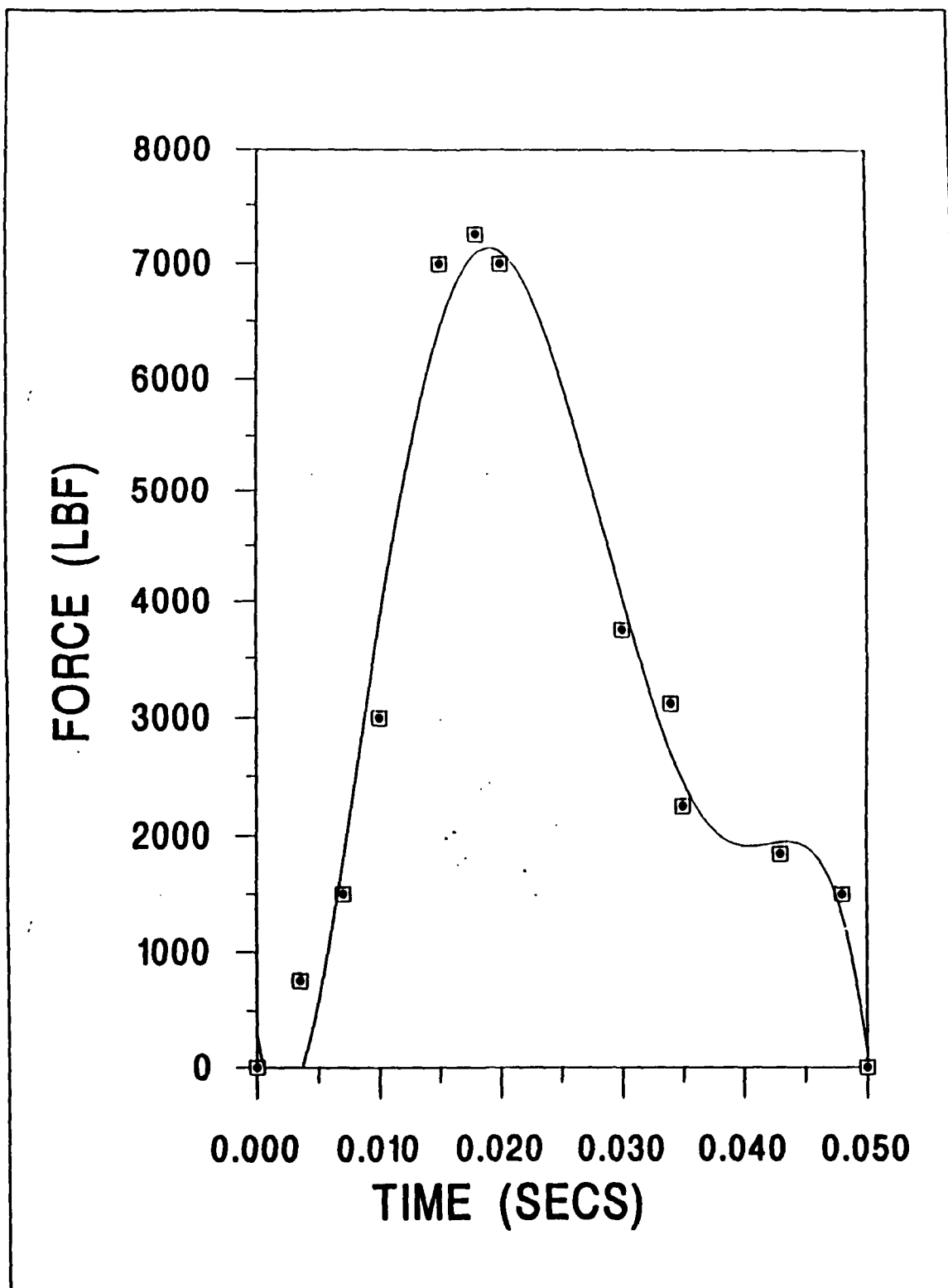
Figure 1 Ejector Force
