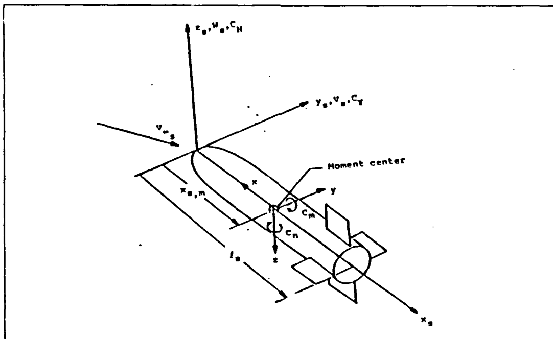
Figure 21 Store Reference Frame
