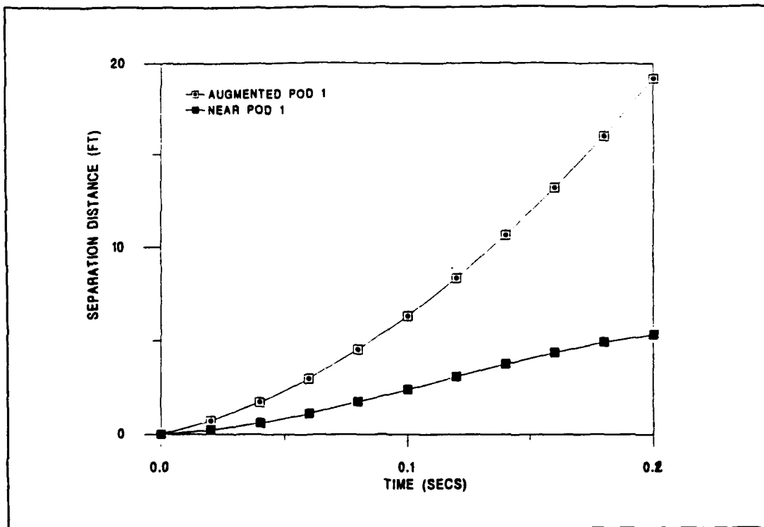
Figure 17 Vertical Separation Distance (Augmented)
