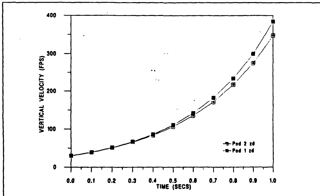
Figure 8 Vertical Velocity
