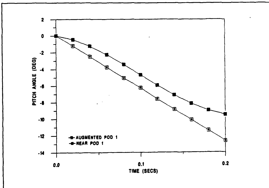
Figure 18 Pitch Angle (Augmented)
