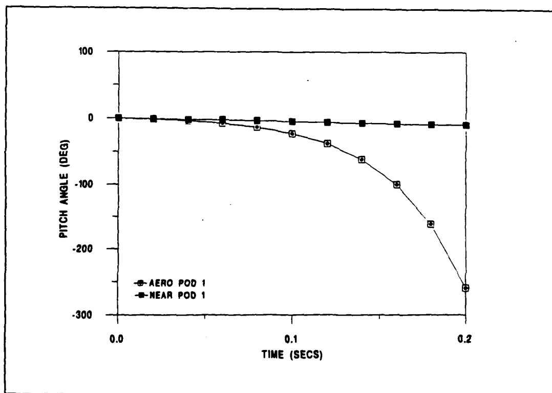
Figure 15 Pitch Angle
