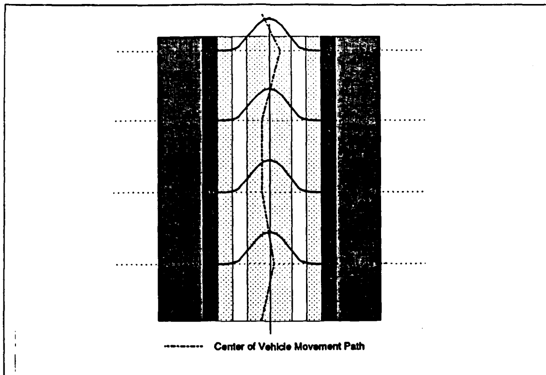
Figure 7. Minefield Path with Driving Errors
