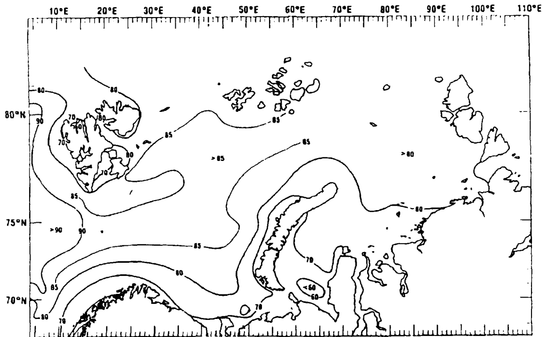
Figure 2.11 Percent frequency of 5/8 or greater coverage by low clouds (< 8000 ft) (NAVOCEANO, 1990).
