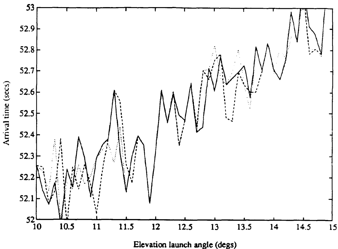
Figure 4.8 Arrival time vs. elevation launch angle for angles from 10° to 15°. Case 1 (Solid), Case 2 (Dashed), Case 3 (Dotted).
