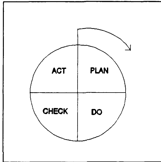
Figure 1: Shewhart Cycle
