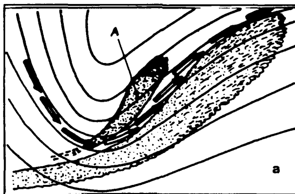
Fig. 14. Baroclinic Leaf Embedded in Upper Level Trough (from Weldon 1979)
