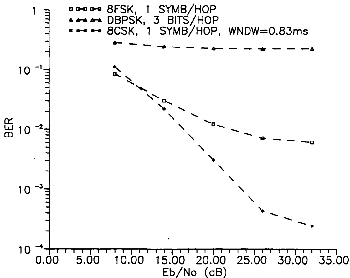
3 Figure 3-4 Performance of 8FSK, DBPSK, & 8CSK for Two Equal-power Rayleigh-Fading Paths, Fading Rate = 10 Hz 3
