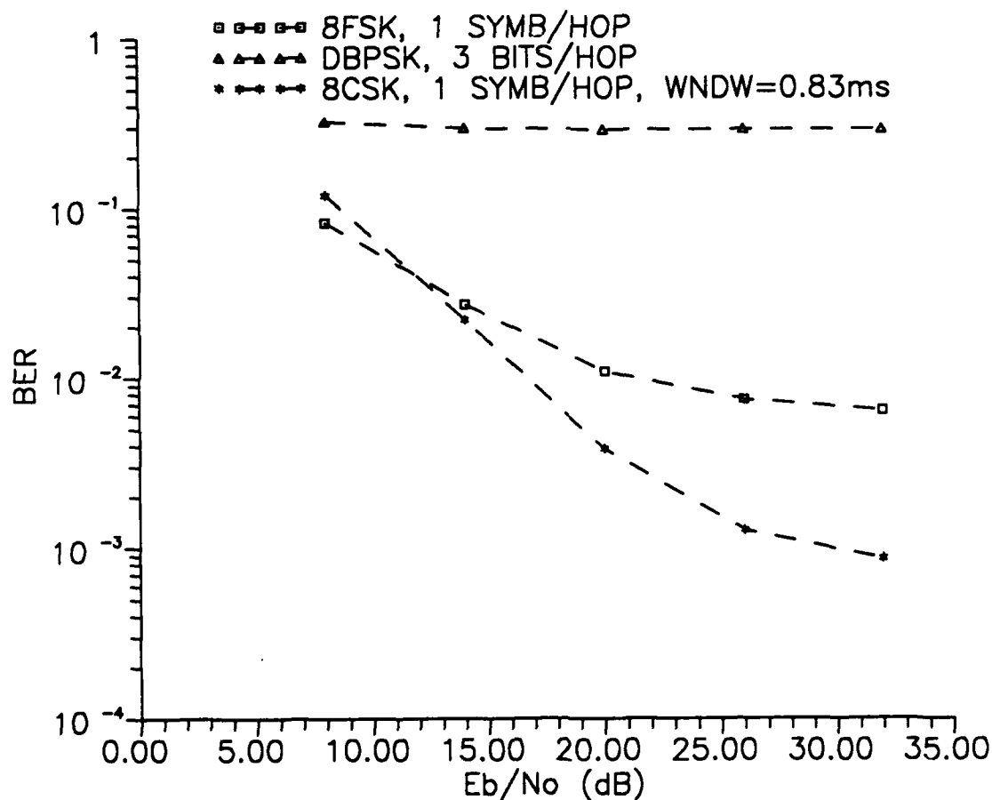
4 Figure 3-3 Performance of 8FSK, DBPSK, & 8CSK for Two Equal-Power Rayleigh-Fading Paths, Fading Rate = 3 Hz 10
