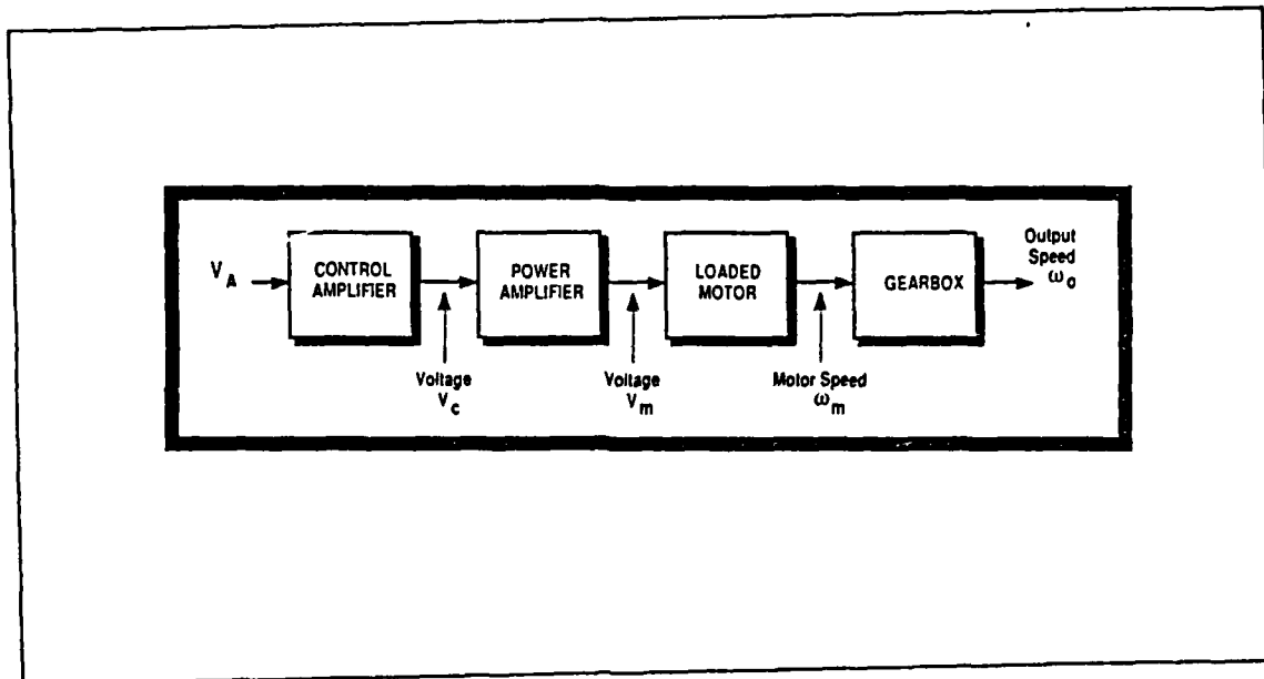
Figure 27. Power and Control Amplifier Block Diagram
