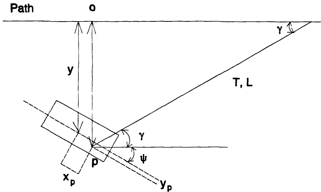
Figure 1. Towed Vessel Coordinate Description.
