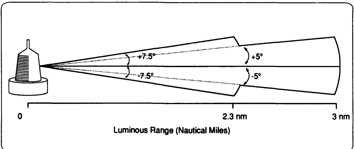
Figure 2. COLREGS Vertical Sector Profile
