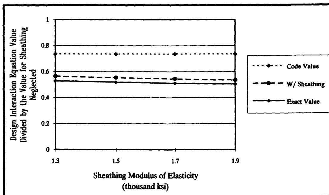
Fig. 3.42 EFFECT OF TRUSS SHEATHING MODULUS OF ELASTICITY ON SHEATHING EFFECTIVENESS FOR INTERACTION EQUATION VALUES (TRUSS 6, MEMBER 13)
