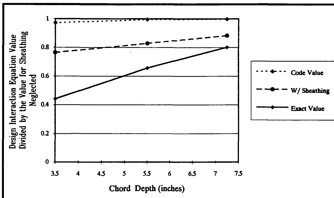
Fig. 3.49 EFFECT OF TRUSS MEMBER DIMENSIONS ON SHEATHING EFFECTIVENESS FOR INTERACTION EQUATION VALUES (TRUSS 1, MEMBER 3)
