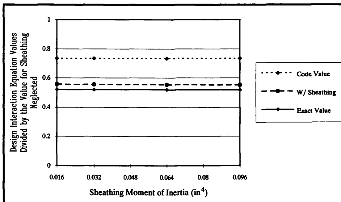
Fig. 3.36 EFFECT OF TRUSS SHEATHING MOMENT OF INERTIA ON SHEATHING EFFECTIVENESS FOR INTERACTION EQUATION VALUES (TRUSS 6, MEMBER 13)
