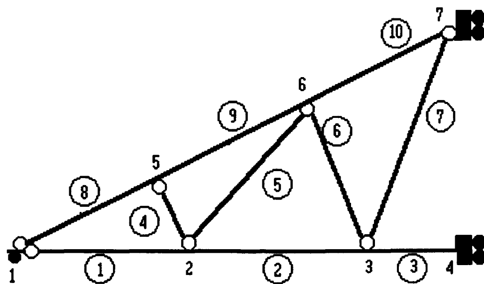
Fig. 3.5 TRUSS 5
