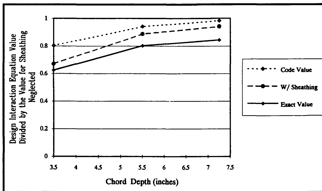
Fig. 3.50 EFFECT OF TRUSS MEMBER DIMENSIONS ON SHEATHING EFFECTIVENESS FOR INTERACTION EQUATION VALUES (TRUSS 2, MEMBER 6)
