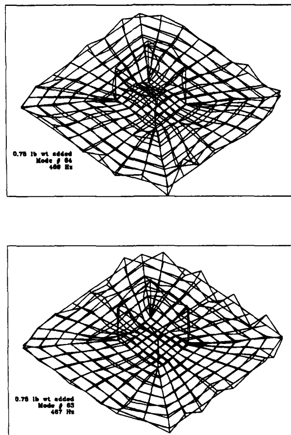
Figure 15. Run # 2 Global Mode Pair
