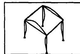
Mode 6 (559 Hz)
