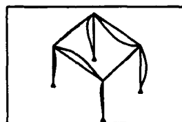
Mode 7 (602 Hz)
