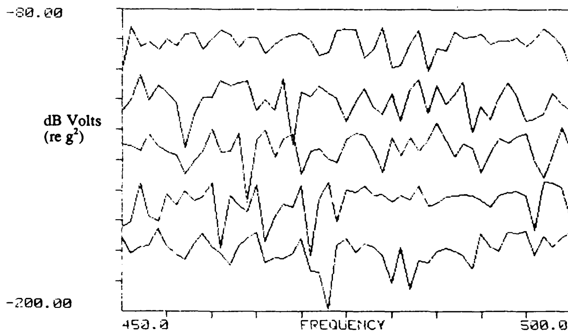
Figure 24. Plate Acceleration for Experiments 1 - 5
