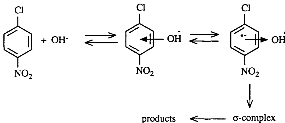
Scheme VII
