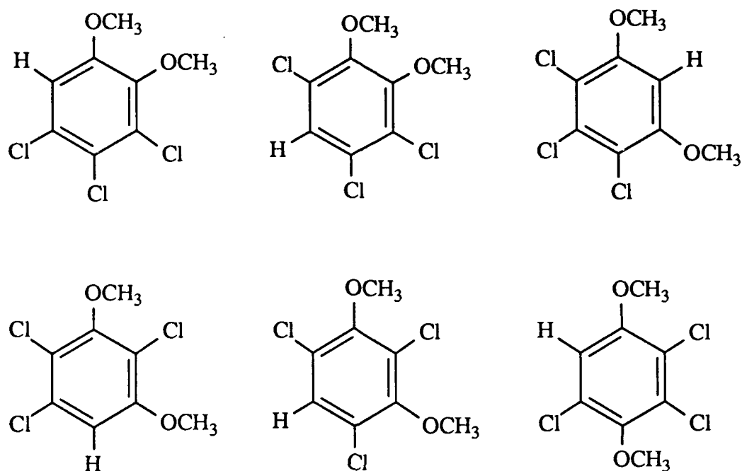
Figure 5. Trichlorodimethoxybenzene Isomers.
