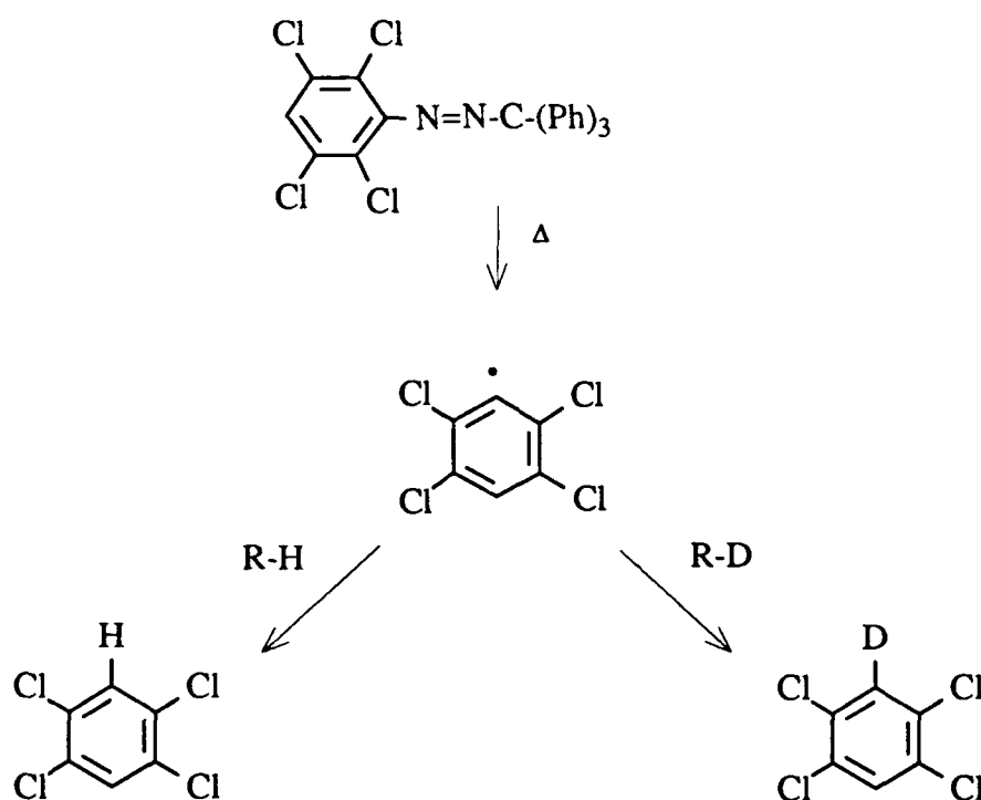
Scheme VIII
