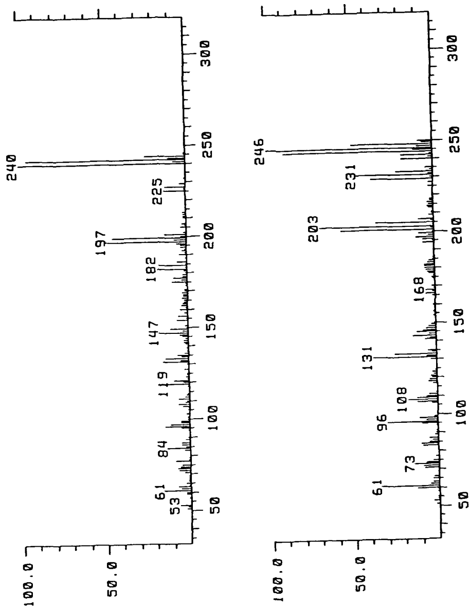
Figure B-2. GC-MS spectra of an isomer of trichlorodimethoxybenzene (TDB, top) and of the ortho -tetrachloroanisole GC peak which contains approximately 10% TDB.
