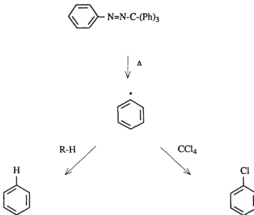
Scheme XIV
