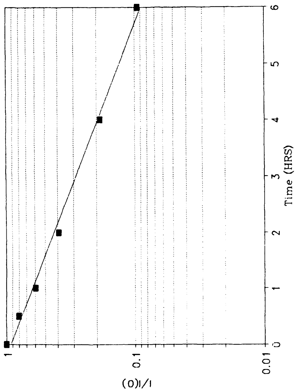
Figure C-4. First-order kinetic plot of the rate of decomposition of TCBAT at 60.0 °C in CCl 4 .
