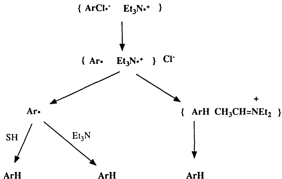
Scheme III
