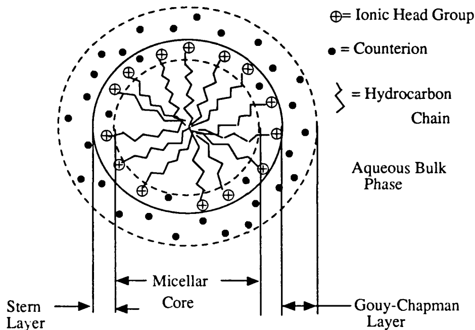
Figure 2. Hartley Model of Micellar Structure.
