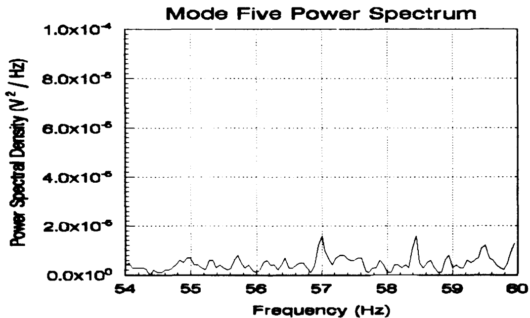
Figure 5.17: Mode five power spectrum.
