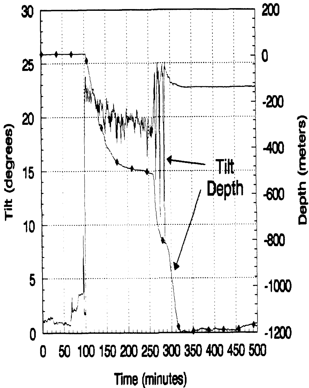
Figure 5.4: Lower sensor output upon deployment.
