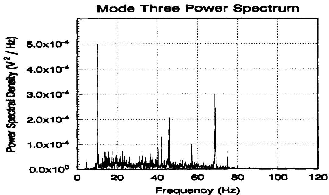
Figure 5.9: Mode three power spectrum.
