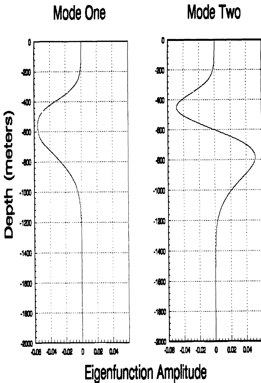
Figure 3.3: Normal modes one and two.
