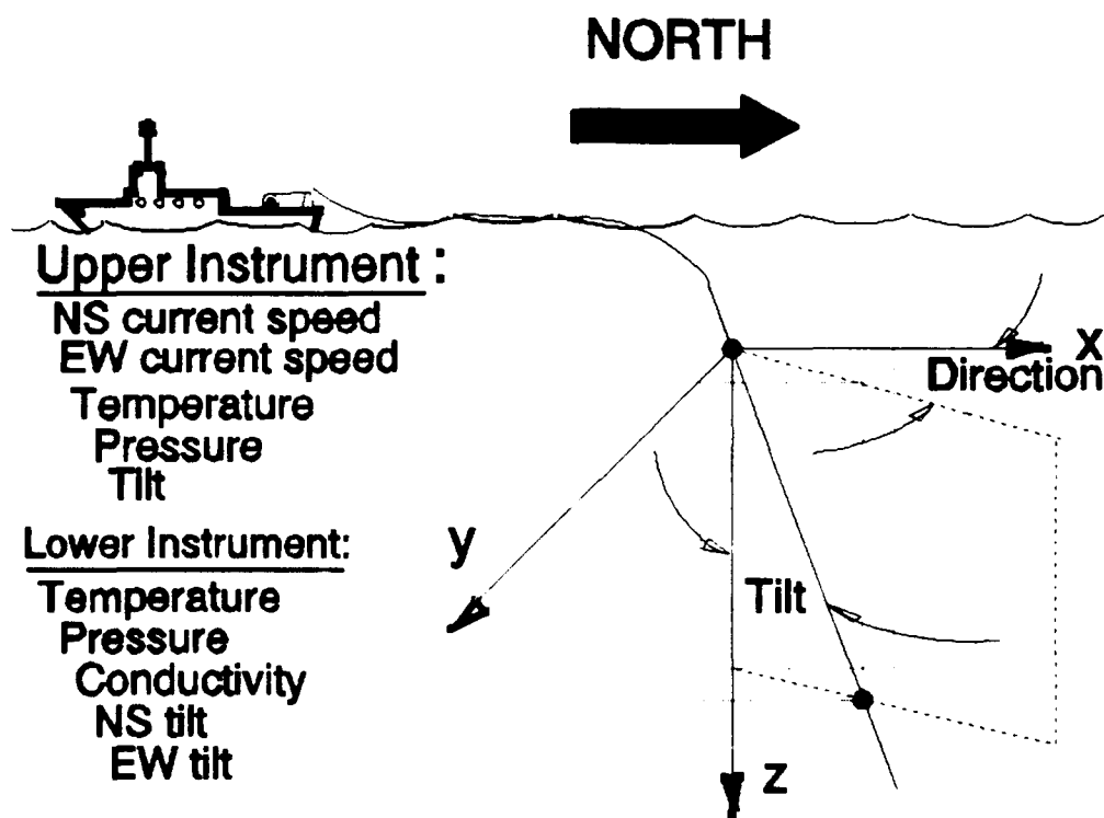
Figure 5.1: Array Instrumentation
