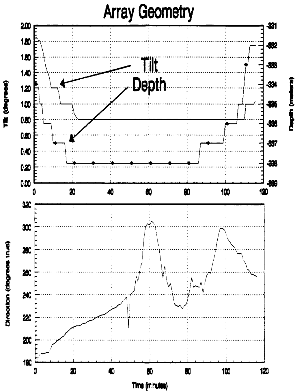
Figure 5.3: Array geometry 15:05 (GMT) January 27.
