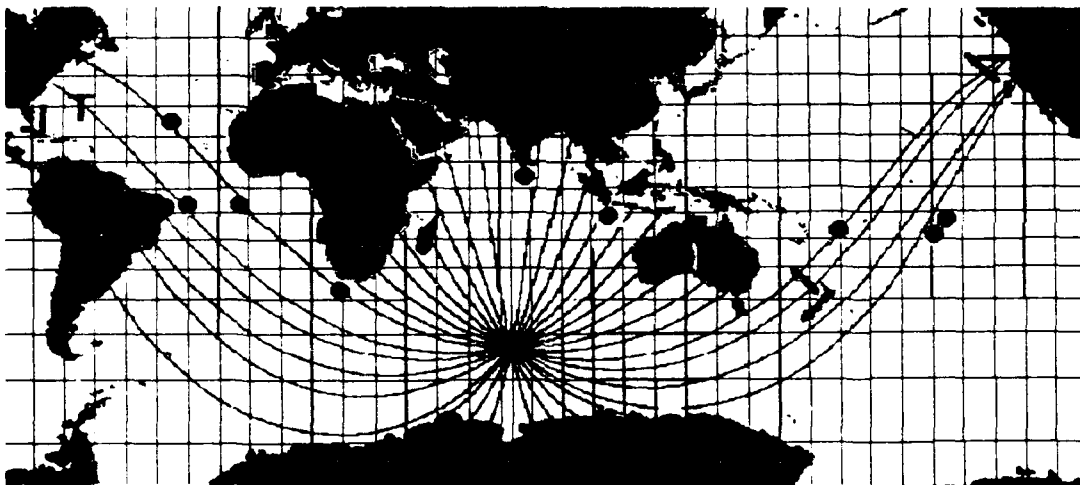
Figure 1.1: Heard Island Raypaths
