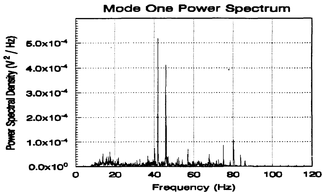
Figure 5.7: Mode one power spectrum.
