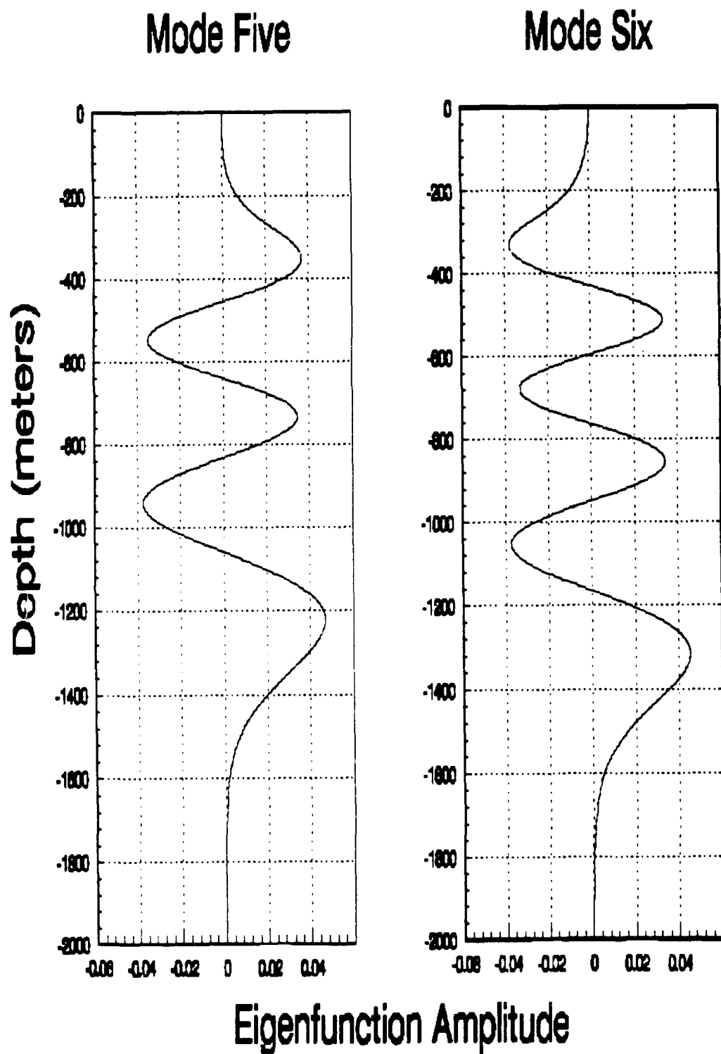
Figure 3.5: Normal modes five and six.
