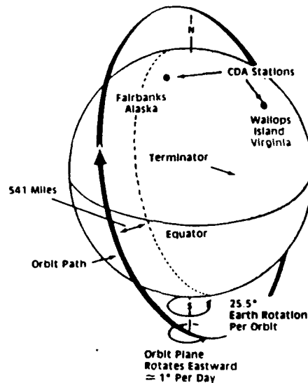
Figure 1: Polar-orbiting Satellites
