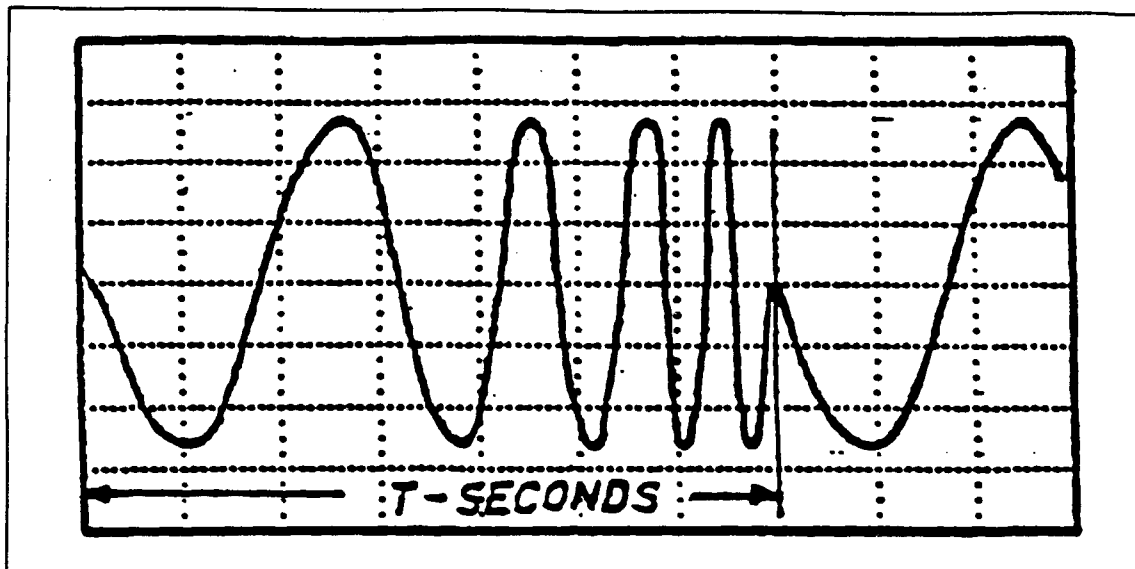
Figure 2 TDS Excitation Signal
