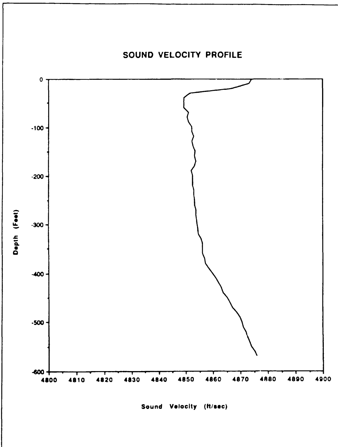
Figure 4 Sound Velocity Profile Taken At Mark 69 Location For Dabob Bay, WA 17 May 1991
