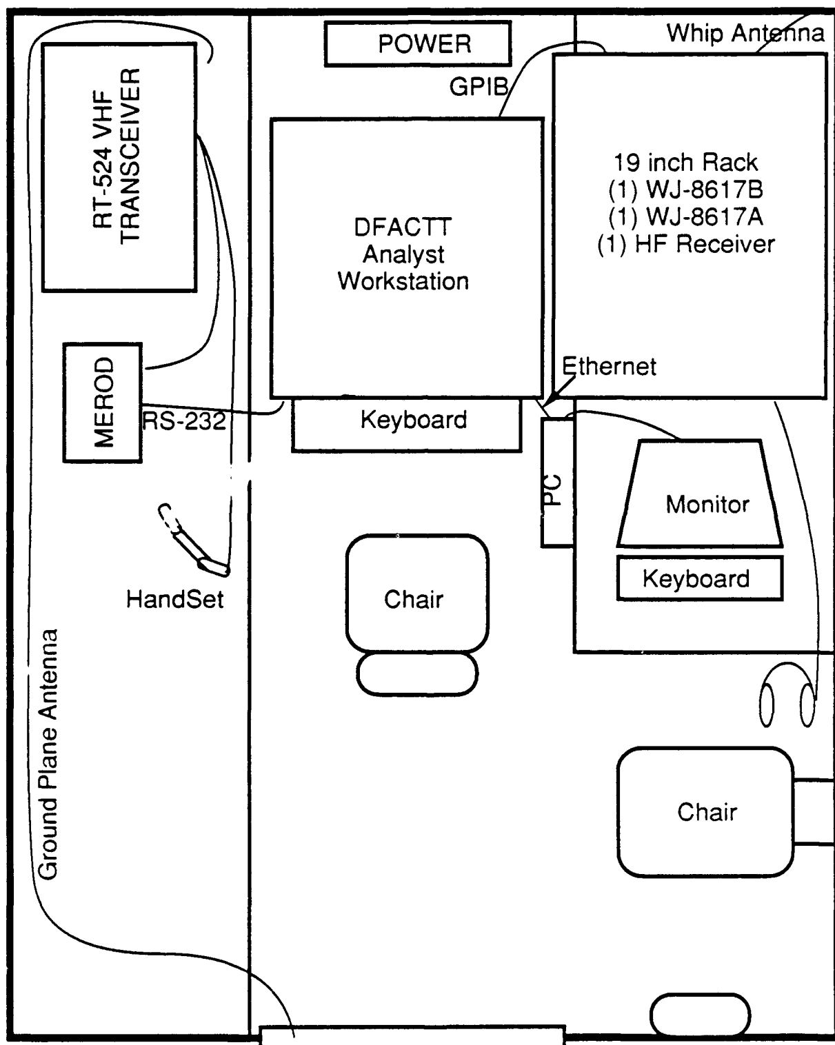
FIGURE A2: DFACTT Layout Inside Vehicle
