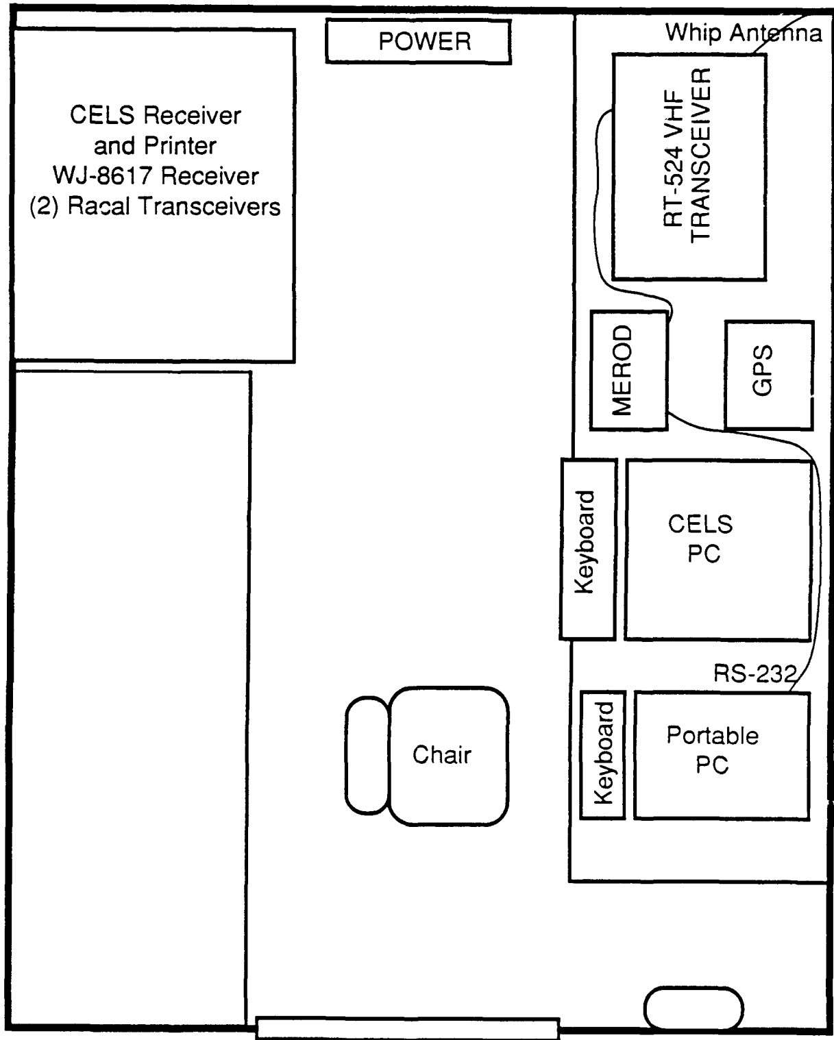
FIGURE A3: Layout of CELS Vehicle
