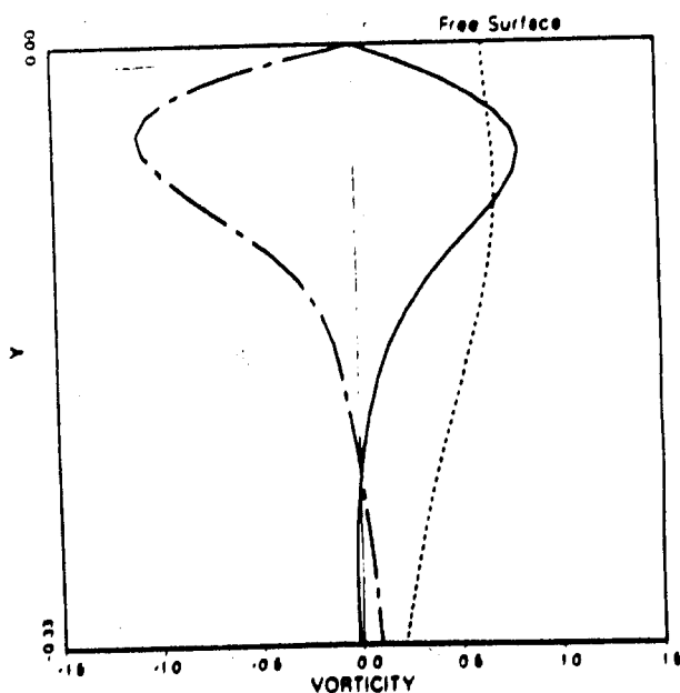
Fig. 7. Ensemble averaged vorticity, conditioned by the requirement that \omega_1\omega_1 \frac{\partial u_1}{\partial x_1} \geq 10\omega_1\omega_1 \frac{\partial u_2}{\partial x_1} . —, \langle \omega_1 \rangle ; ---, \langle \omega_2 \rangle ; ----, \langle \omega_3 \rangle .
