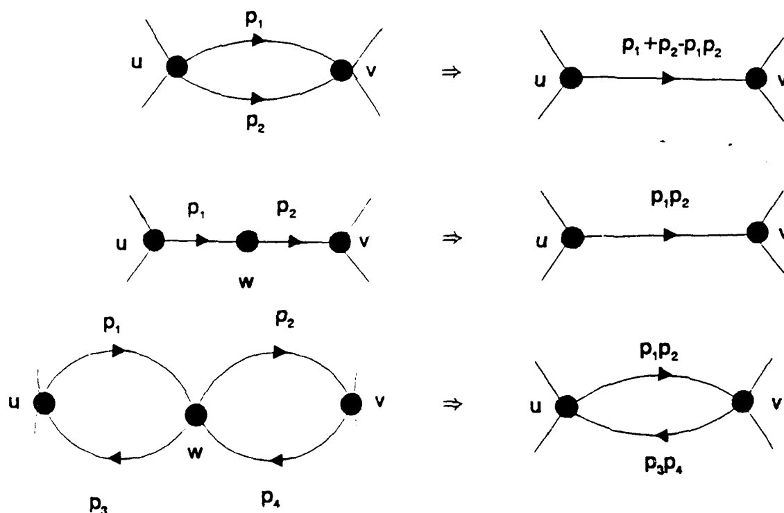
FIGURE 6.5 PARALLEL AND SERIES EDGE REDUCTION ( w \neq s, t )
