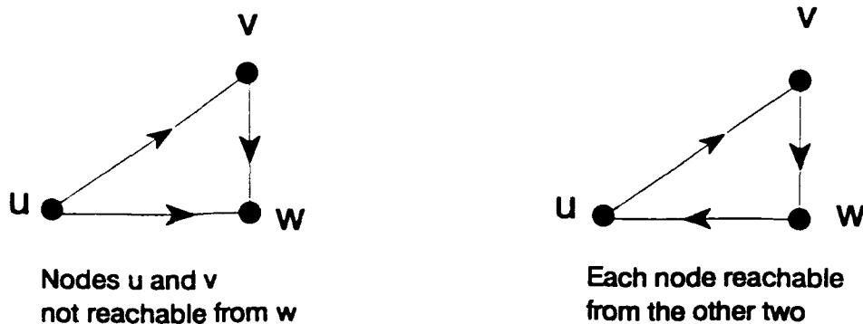
FIGURE 3.2 STRONGLY DISCONNECTED AND CONNECTED
