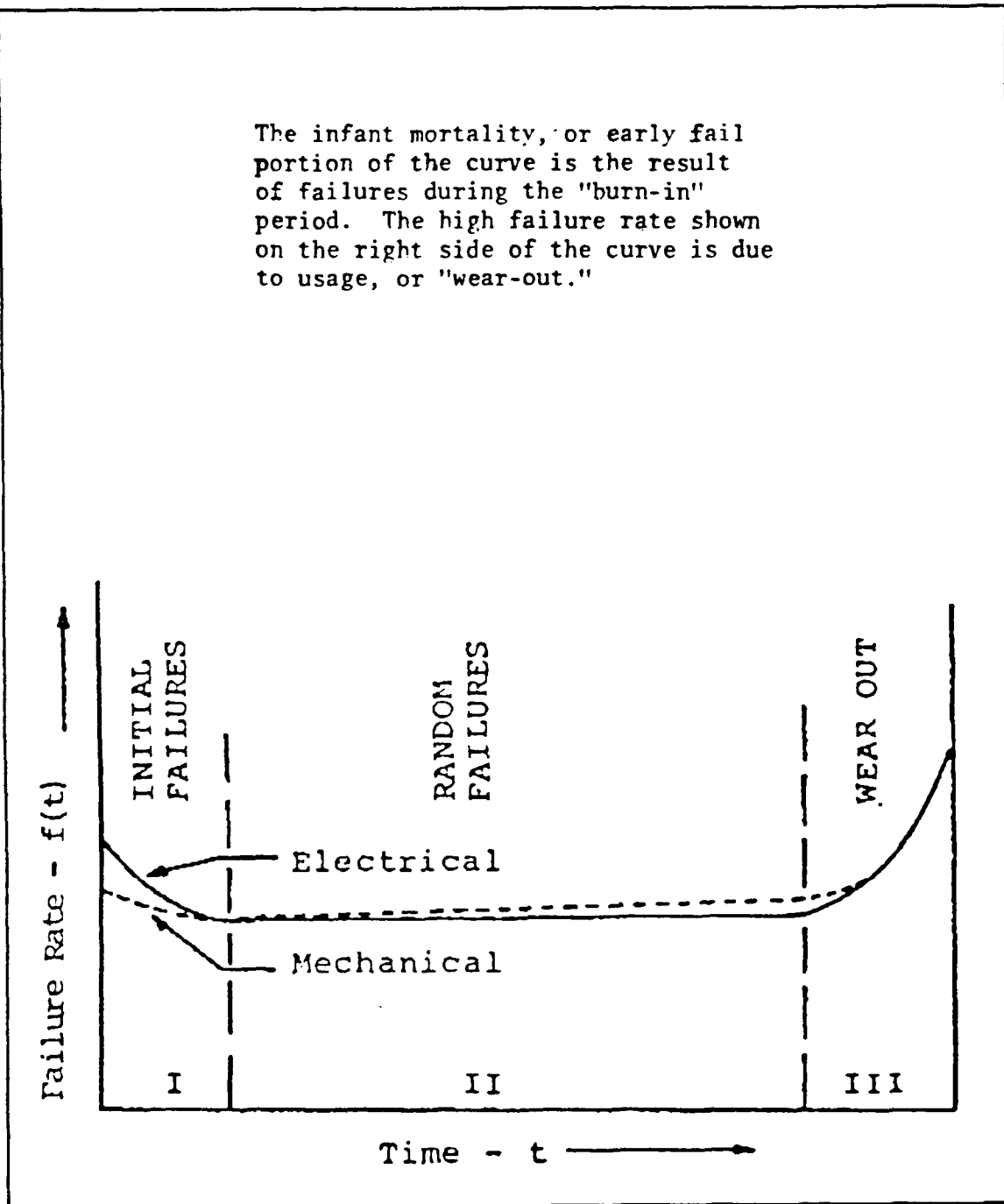
Figure 2. Failure rate as a function of time for typical component. Source: Reference 3.
