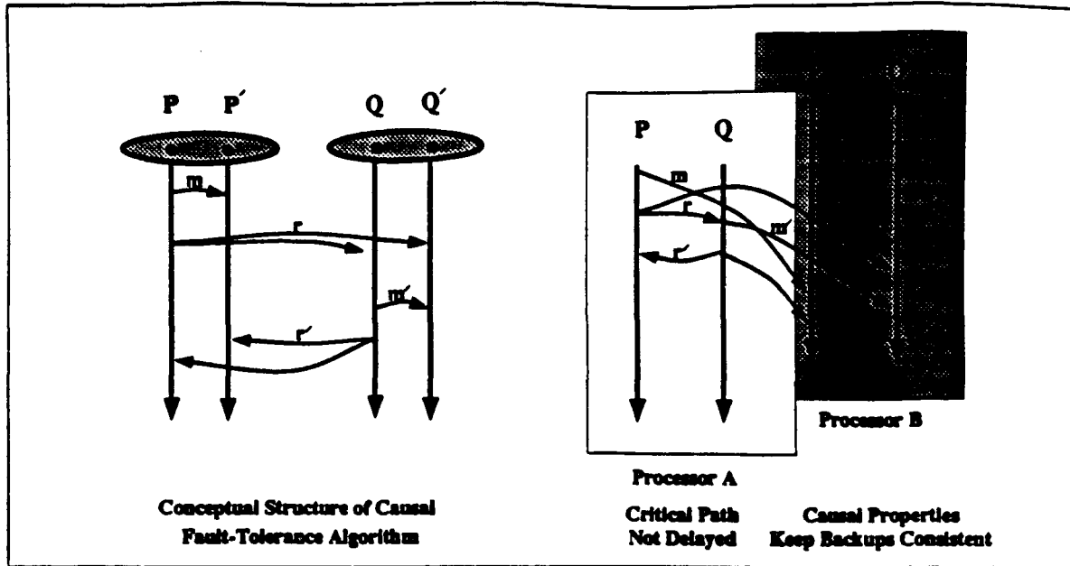
Figure 6: Transparent fault-tolerance using causal process-groups.
