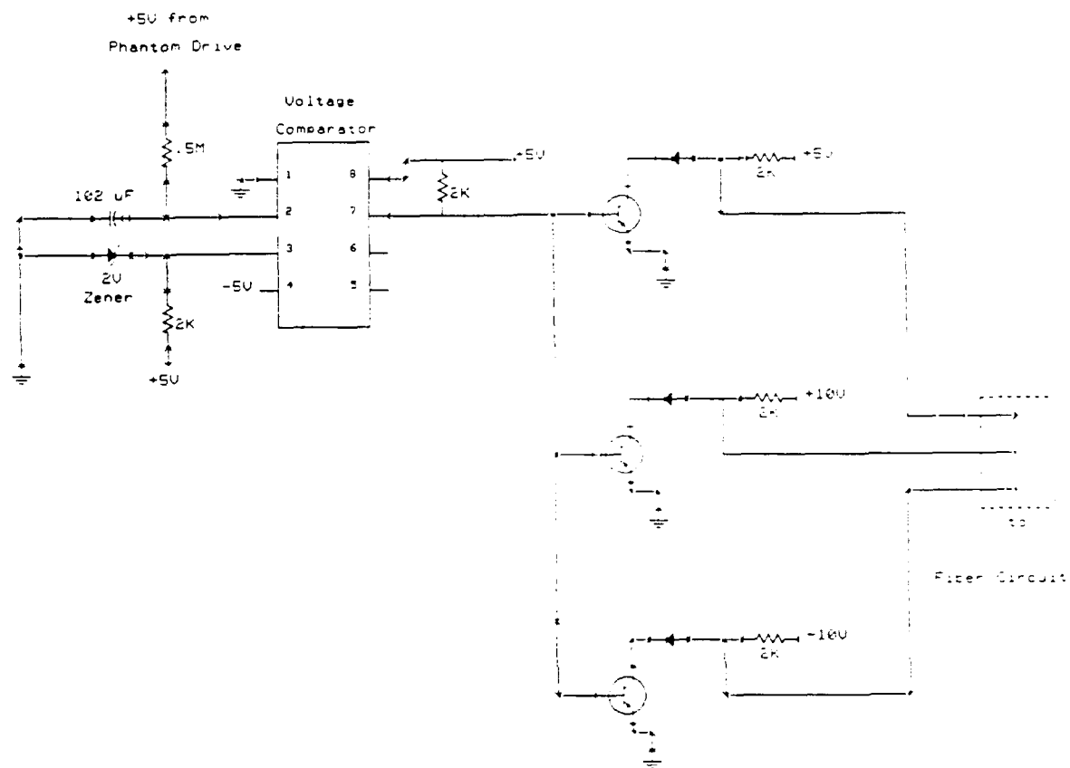
Figure 4-10. Schematic Diagram of Power Switch
