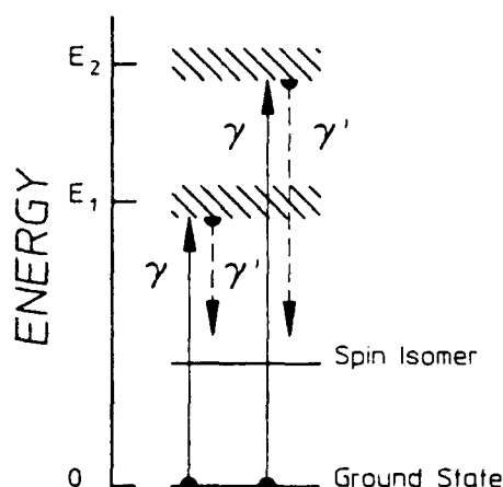
FIG. 1. Schematic representation of the (\gamma, \gamma') reactions used to populate isomeric states in these experiments. The resonant absorption of bremsstrahlung x rays, denoted as \gamma , excite populations of gateway states. Two are shown at excitation energies of E_1 and E_2 but the actual number will vary for each nuclide. Parts of the populations of the gateway states make transitions to the final state either directly or as part of a cascade of radiative transitions ending on the final state as indicated by the dashed arrows.
