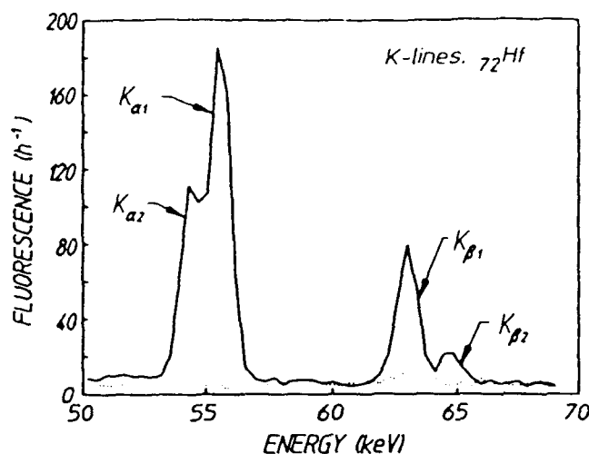
FIGURE 4.5.4 Dotted and solid curves show, respectively, the spectra obtained before and after dumping some of the isomeric ^{180\text{m}}\text{Ta} contained in a target sample enriched to 5%. An HPGe detector was used to obtain the dotted spectrum before irradiation. The feature at 63 keV is from traces of natural activity in the counting shield. The solid curve is the spectral signature of the radioactive debris accumulated by cascading from the levels into which the isomeric population was dumped. The actual lines are the K-lines of hafnium arising from electron capture by the ^{180\text{m}}\text{Ta} ground debris.
