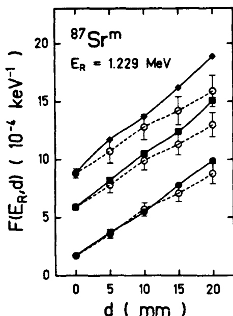
FIG. 1. Comparison of the photon flux at resonance energy E_R to the 1.332-MeV line flux for different geometries of a ^{60}\text{Co} source. The characteristic ratio F(E_R, d) is shown as a function of the Pb scatterer thickness for a pointlike source (open circles), an extended source (solid circles), an extended source plus 1-cm Pb shielding (squares), plus 2-cm Pb shielding (diamonds). For details of the extended source geometry, see text. Statistical errors of the extended source calculations (not shown) are of the order of the symbol size. The straight and dashed lines are drawn to guide the eye.
