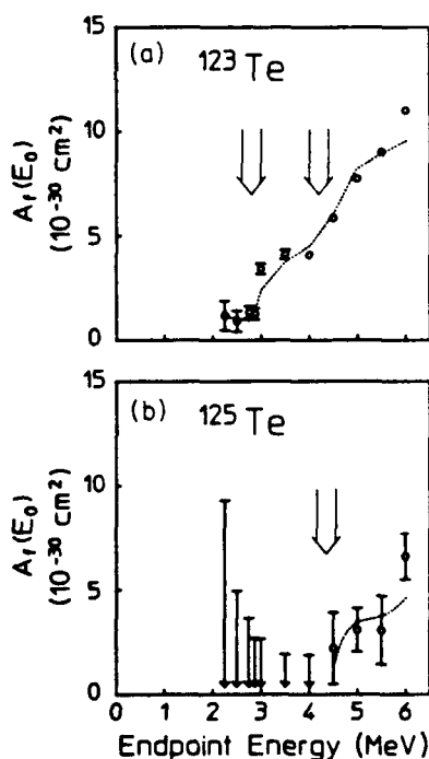
FIG. 3. Linear plots of yield normalized to the flux calculated for a low-energy cutoff of 1 MeV as functions of bremsstrahlung end-point energy for (a) ^{123}\text{Te} and (b) ^{125}\text{Te} . Where no error bars are shown, statistical errors are comparable to the symbol size. Error bars shown without symbols in (b) represent upper bounds on the activation where fluorescence was not observed above the level of background. Dotted curves plot the values calculated from the model of Eq. (4) using the results of Table I. The locations of the gateways determined in this work are indicated by the large arrows whose widths represent the available experimental resolution.
