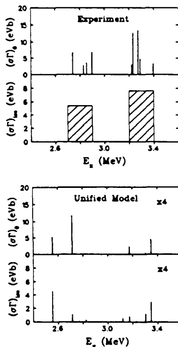
Fig. 3. Comparison of the experimental (\sigma\Gamma)_0 and (\sigma\Gamma)_{\infty} results with unified-model calculations. The dashed histograms for the experimental (\sigma\Gamma)_{\infty} strength indicate that they might be the sum of unresolved states within the experimental resolution.
