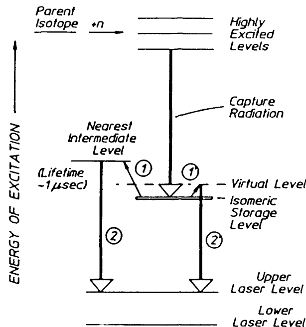
FIGURE 4 5 1 Schematic diagram showing the energetically excited levels of a typical nucleus of interest to the development of a gamma-ray laser. Life-times of the stored energies in the isomeric level produced by the initial capture can range from days to hundreds of years. The first phase of the two-step process for the stimulated release of the stored energy is shown in the figure by the solid arrows. Both subsequent alternatives correspond to the use of longer wave-length radiation to lift a nucleus from the storage level to a higher level of excitation that has a much shorter lifetime. The arrow marked (1) illustrates the incoherent pumping of the storage level through the absorption of an x-ray that is resonant with the energy separation between the storage level and the next higher level of proper symmetry. The arrow marked (1') represents the alternative process of coherent pumping through the nonresonant absorption of a photon from the radiation field in order to create a virtual or dressed state of excitation shown by the dashed level in the figure. In either case the gamma-ray output ultimately results from the upper laser level populated by a cascade occurring as a second step, as shown in the figure by either of the double arrows, (2) and (2').
