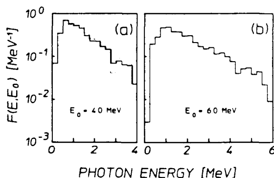
FIG. 3. Relative spectral intensities F(E, E_0) of the bremsstrahlung produced by the medical linacs used to irradiate samples in these experiments. The curves are normalized so that their areas are unity. The solid lines indicate empirical fits to the calculated spectra as discussed in the text. The devices employed were as follows: (a) Varian Clinac 4/100, with a nominal end point of 4 MeV. The dotted curve shows the spectrum obtained from Ref. 21 that contains a computational artifact at about 3 MeV. (b) Varian Clinac 1800, operated in the nominal 6 MeV end-point mode.
