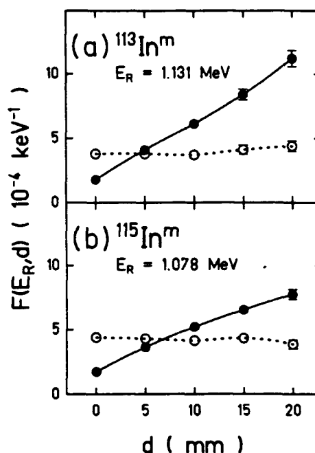
FIG. 2. Direct (solid circles) and scattered (open circles) contributions to F(E_R, d) from the simulation of the experiments described (a) in Ref. [4] and (b) in Ref. [2]. For details, see text. The straight and dashed lines are drawn to guide the eye.
