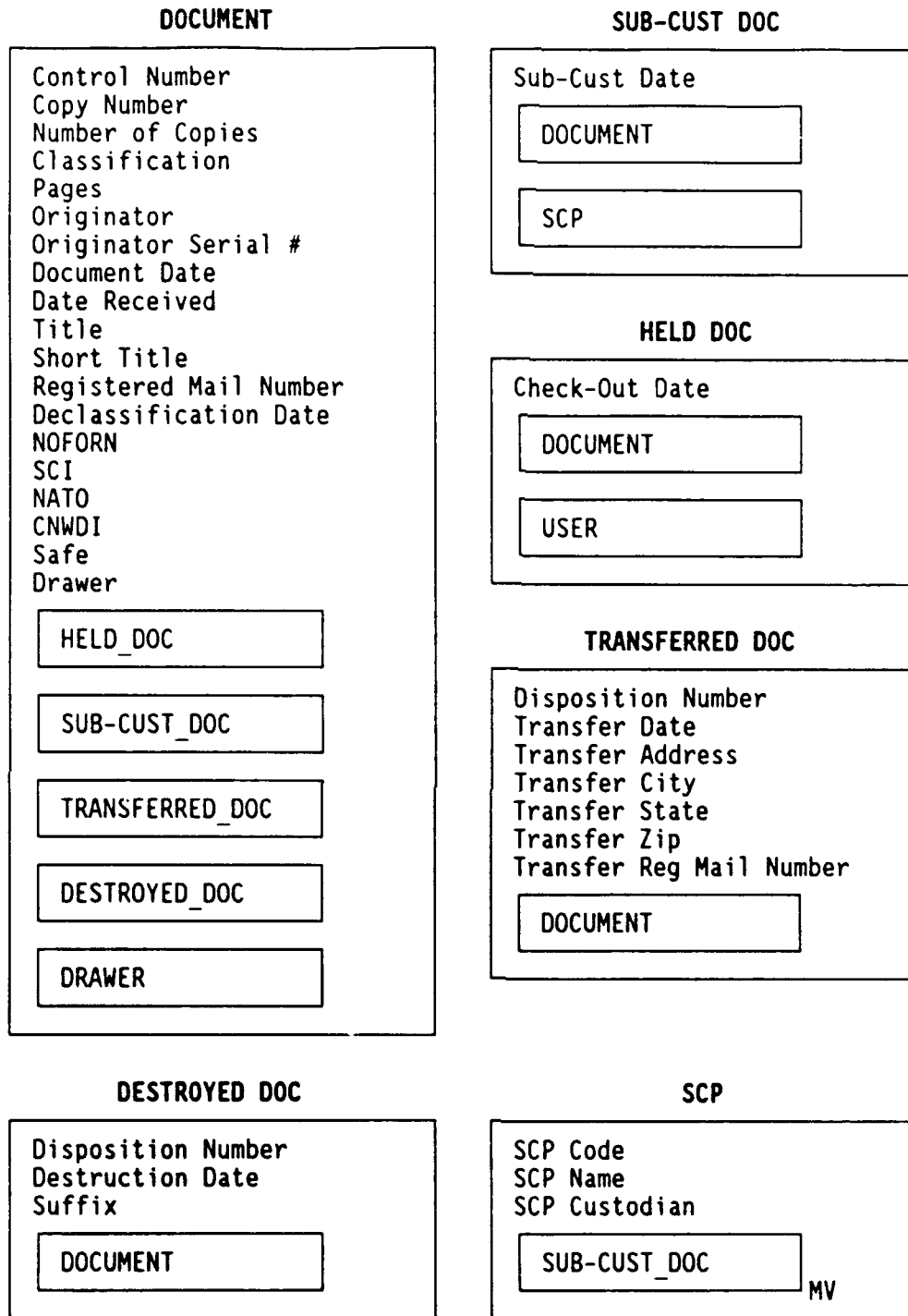
Figure 7. Object Diagrams.
