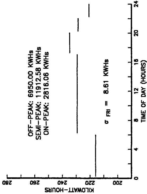
FRIDAY (BILLING PERIOD 5) AVG. KWH DATA
